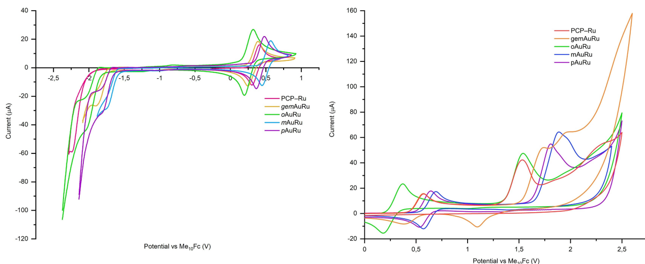
Figure 11. Cyclic voltammograms of PCP-Ru ( 22 ) and AuRu isomers 6 and 18–20 (left) and CV spectra of the second oxidation process (right) ( 0.1 M \text{Bu}_4\text{NPF}_6 , \text{CH}_2\text{Cl}_2 , 100 mV/s).
