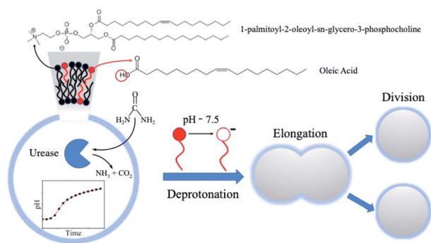
Fig. 1 Schematic representation of the self-division process of GUVs. Mixed POPC/HOA ([POPC]/[HOA] = 2.6 mM/2.4 mM) vesicles containing the enzyme urease were prepared by a phase transfer method. Urea was added to the external solution to trigger the reaction inside the lumen of the vesicles. Following the urea trans -membrane permeation, the pH increase causes the deprotonation of the oleic acid in the inner leaflet of the bilayer, which, in turn, induces vesicle division.
