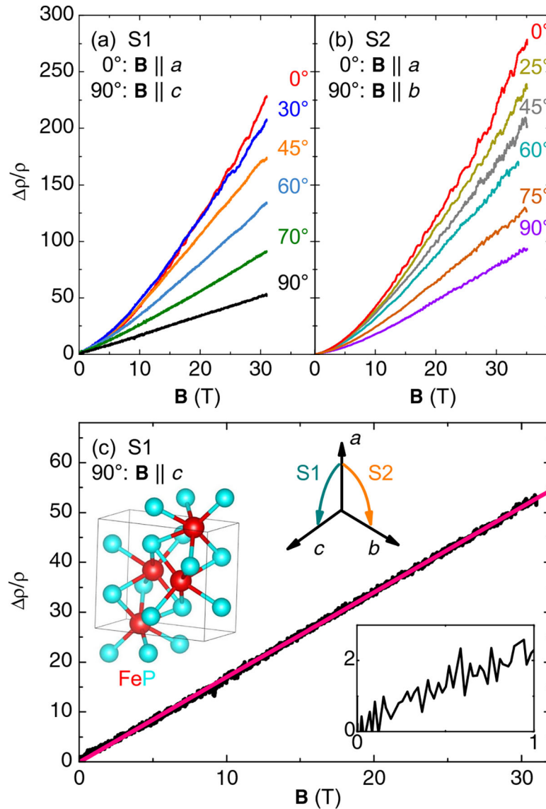
Fig. 2. Magnetoresistance of FeP at high field.
