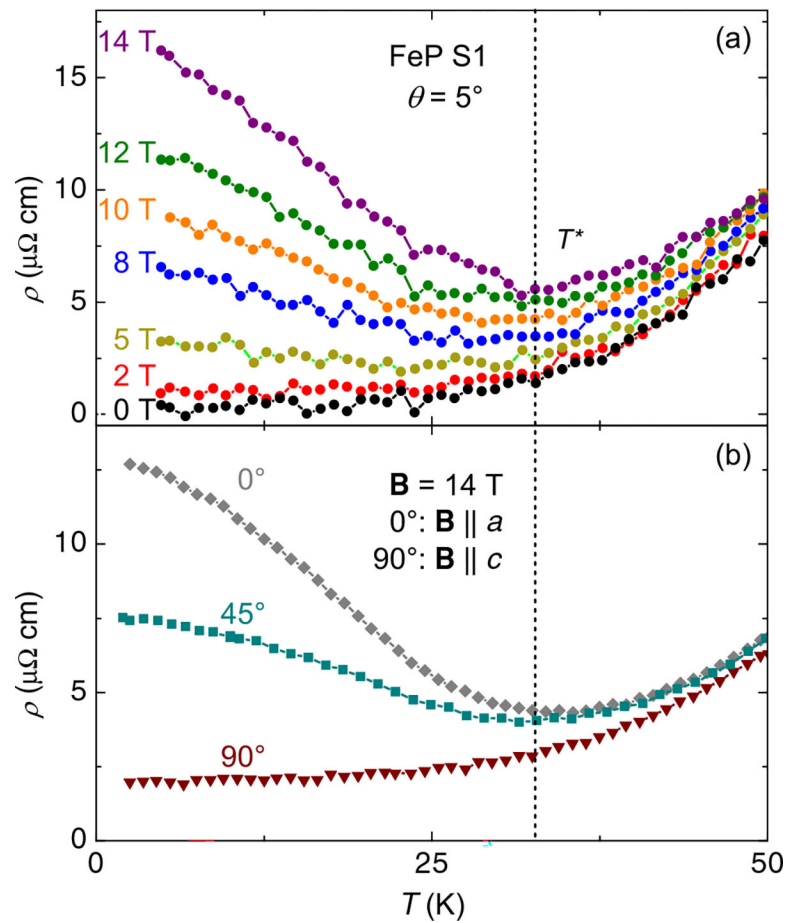
Fig. 4. Temperature dependence of sample S1 for different magnetic field strengths and orientations.
