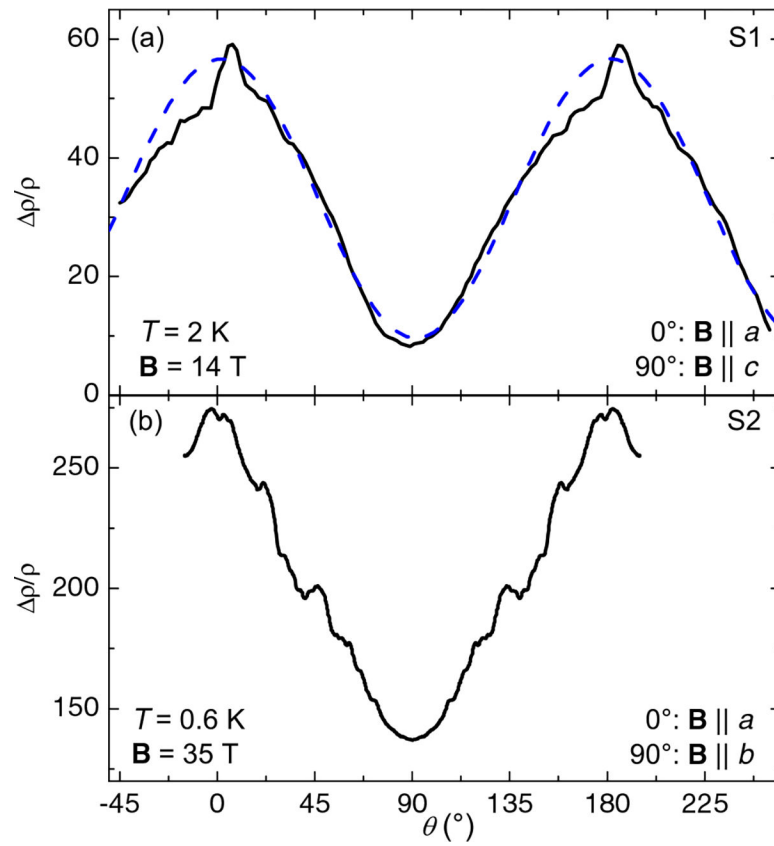
Fig. 3. MR as a function of angle at constant field.
