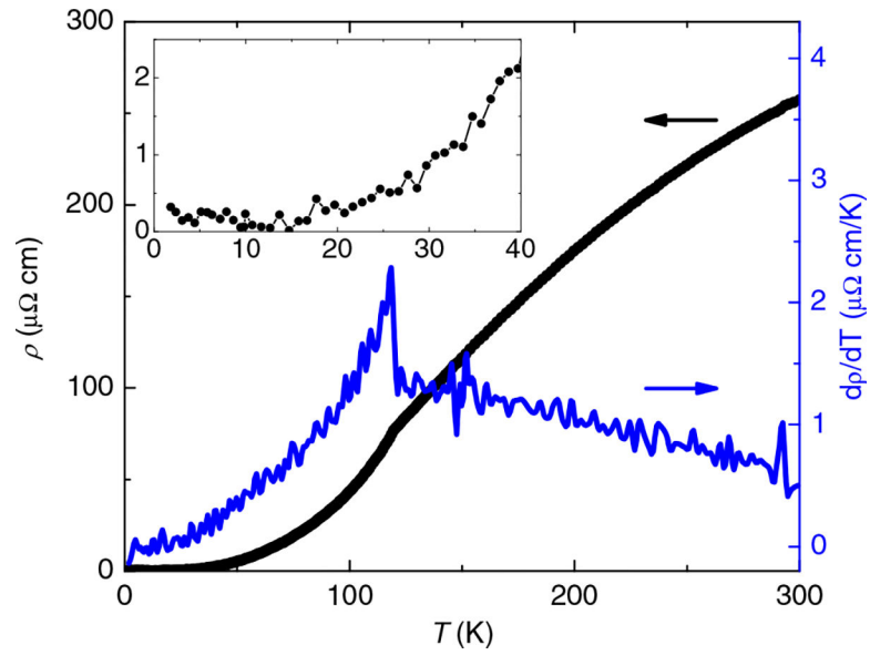
Fig. 1. Temperature dependence of the resistivity of FeP.
