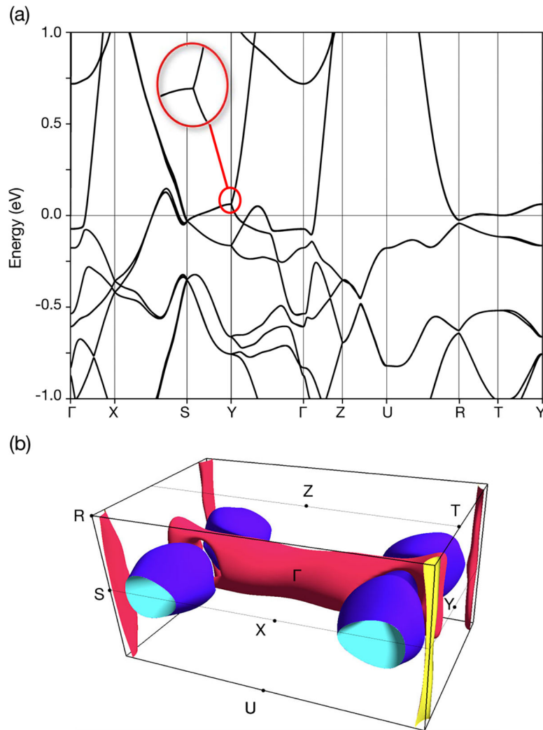
Fig. 5. Density functional theory results for FeP.
