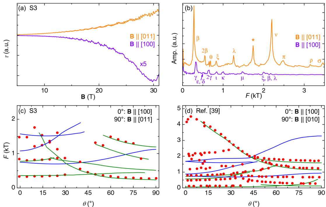
Fig. 6. Experimental-theoretical comparison of quantum oscillations.
