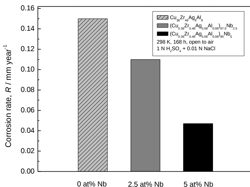
Figure 13. Average corrosion rates of the as-cast (\text{Cu}_{0.36}\text{Zr}_{0.48}\text{Ag}_{0.08}\text{Al}_{0.08})_{100-x}\text{Nb}_x ( x = 0\text{--}5 at.%) alloys in 1 N \text{H}_2\text{SO}_4 + 0.01 \text{ N NaCl} solution at 298 K open to air.
