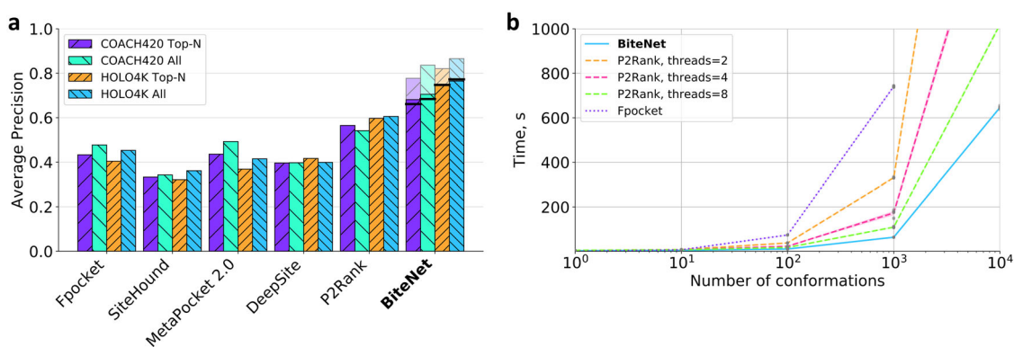
Fig. 6 Predictive power and computational efficiency of BiteNet. a Performance of the binding site prediction methods on the COACH420 and HOLO4K benchmarks. Violet and orange bars with diagonal hatching correspond to the average precision calculated for top N predictions for the COACH420 and HOLO4K benchmarks, respectively, where N is the number of true binding sites in a protein. Similarly, cyan and blue back hatched bars correspond to the average precision calculated for all predictions for the COACH420 and HOLO4K benchmarks, respectively. Pale bars correspond to the BiteNet performance, when the true positive binding site is defined as in the training. Black lines correspond to the BiteNet performance on the whole benchmarks. b Elapsed time for fpocket (dotted violet line), P2Rank (dashed orange, magenta, and green lines), and BiteNet (solid blue line) to analyze 1, 10, 1000, and 10,000 conformations of a protein with \sim 2000 atoms. The computed elapsed time is the average of ten independent runs, individual data points are shown with gray circles.
