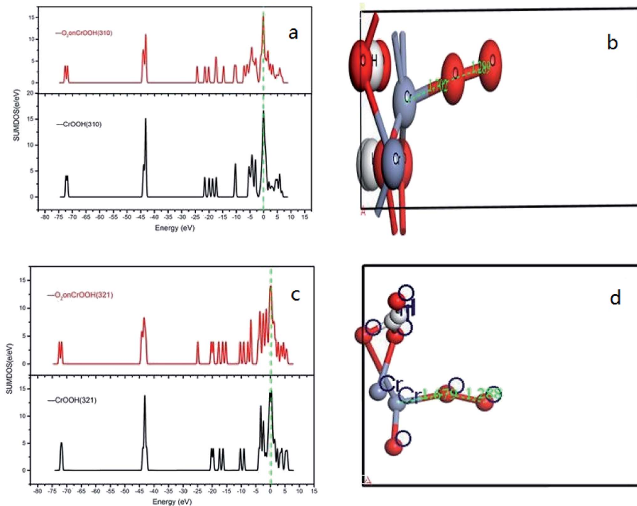
Fig. 13 (a) the total density of states of CrOOH (310) surface adsorption model; (b) the side view of optimized CrOOH (310) surface adsorption model; (c) the total density of states of CrOOH (321) surface adsorption model; (d) the side view of optimized CrOOH (321) surface adsorption model.
