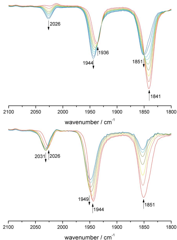
Fig. 4 IR-SEC of \mathbf{11} : top: E = 0.21 V \mathbf{11} (red) to \mathbf{11}^+ (blue). Bottom: E = 0.45 V \mathbf{11}^+ (red) to \mathbf{11}^{2+} (blue).
