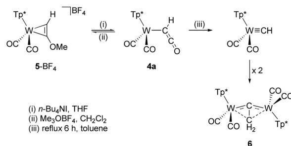
Scheme 2 Reversible alkylation of 4a and \text{CO} release.
