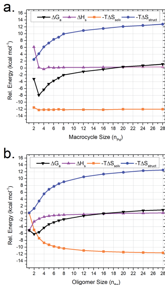
Fig. 4 MD-calculated thermodynamic parameters for (a) M_n^{\text{lin}}L_n macrocyclic and (b) M_n^{\text{lin}}L_{n+1} oligomeric assemblies. Energy values are plotted on a common scale where -T\Delta S_{\text{solv}} and -T\Delta S_{\text{struct}} contributions are plotted relative to M_1^{\text{lin}}L_2 while \Delta H is plotted relative to M_{28}^{\text{lin}}L_{29} . The sum of -T\Delta S_{\text{solv}} , -T\Delta S_{\text{struct}} and \Delta H values is plotted as \Delta G .
