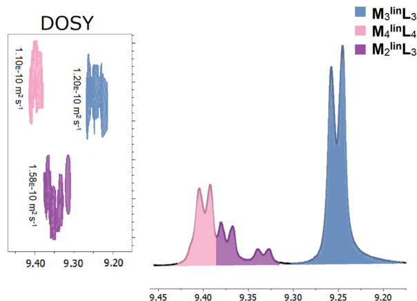
Fig. 1 Macrocylic and oligomeric products observed from the self-assembly of M (17.1 mM) and linL (17.1 mM) in DMSO characterized by unique \alpha -pyridyl peaks in ^1\text{H-NMR} (Fig. S1†), with inset DOSY (Fig. S2†) diffusograms. Three distinct assemblies were observed and high-lighted for clarity: \text{M}_3^{\text{linL}_3} (slate blue), \text{M}_4^{\text{linL}_4} (pink), and \text{M}_2^{\text{linL}_3} (purple). Numerical data is provided below in Table 1.
