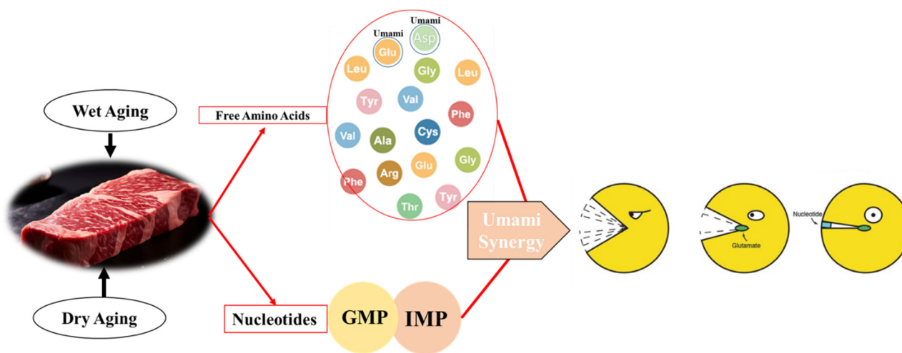
Fig. 2. The umami and other taste perception mechanism. Adapted from Schmidt and Mouritsen (2022) with CC-BY-NC-ND. GMP, guanosine monophosphate; IMP, inosine monophosphate.
