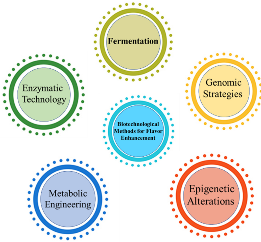
Fig. 4. The cutting-edge biotechnological methods for flavor development.
