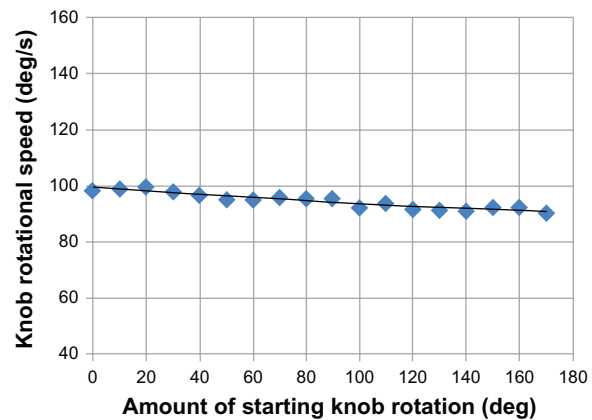
Figure 11 Bottom knob rotational speed.
