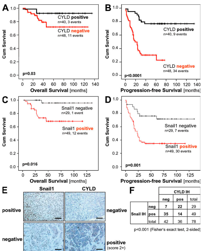
Figure 7. CYLD expression in melanoma has prognostic implications. Kaplan-Meier curves for overall survival (A) and progression-free survival (B) in melanoma patients with a positive immunosignal for CYLD (CYLD positive) or without detectable CYLD protein expression (CYLD negative). CYLD immunohistochemical staining of primary malignant melanoma tissue was performed using a tissue microarray consisting of 88 cases. Investigation of CYLD protein expression was informative in all specimens. Kaplan-Meier curves for overall survival (C) and progression-free survival (D) in melanoma patients with a positive immunosignal for Snail1 (Snail1 positive) or without detectable Snail1 protein expression (Snail1 negative). Snail1 immunohistochemical staining of primary malignant melanoma tissue was performed using a tissue microarray consisting of 88 cases. Immunohistochemical analysis of Snail1 was informative in 78 samples. (E) Examples of tissues with positive and negative CYLD and Snail1 staining, respectively. Bar, 100 \mu m. (F) Comparison of CYLD and Snail1 immunoreactivity. An inverse correlation of CYLD and Snail1 staining was observed.
