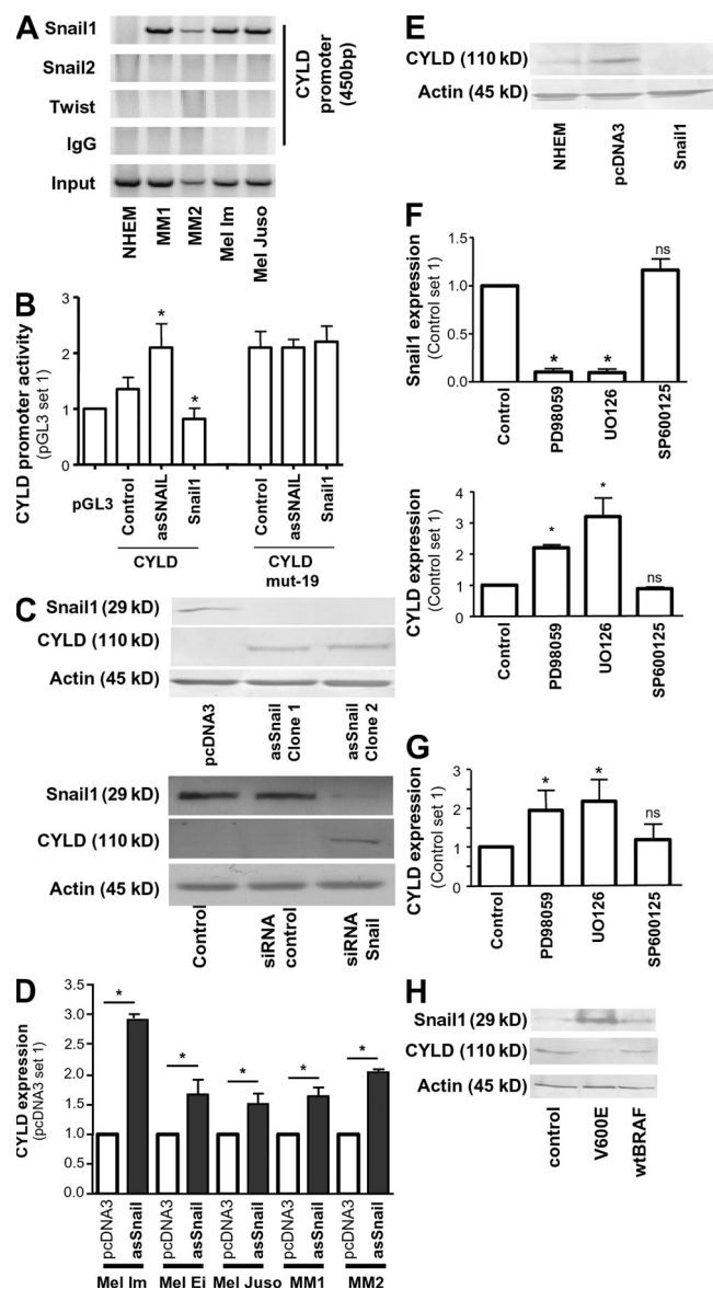
Figure 2. Snail1 inhibits transcriptional expression of CYLD in melanocytic cells. (A) Lysates from NHEMs, primary melanoma cells (MM1 and MM2), and melanoma cell lines (Mel Im, Mel Juso) were examined by ChIP assay using an anti-Snail1, anti-Twist, and anti-Snail2-specific antibody, respectively, as well as a PCR primer pair corresponding to the promoter of the CYLD gene. Recruitment to the CYLD promoter was only shown for Snail1. Snail1, Twist, Snail2, immunoprecipitation (IP) using specific antibodies; IgG, IP using negative control rabbit immunoglobulin; Input, 10% of the cell lysate used for the IP is shown. (B) Reporter assays revealing inducible CYLD promoter (−550 to −1 bp) activity in Mel Im cells after transient transfection with asSnail (asSnail), whereas transfection with Snail1 expression plasmid (Snail1) completely abrogated CYLD promoter activity compared with the control (pGL3). Mutation of the consensus Snail1 binding site ( CYLD mut-19) led to strong promoter activity that was not affected by transfection with asSnail or Snail1. Data are given as mean ± SEM. *, P < 0.05 compared with CYLD control. (C) Immunoblot analysis showing that CYLD protein is up-regulated in Mel Im cells after stable transfection with asSnail expression plasmids (clone 1 and clone 2; top) and after transient transduction with Snail1 siRNA nucleotides (siRNA Snail1) or scrambled siRNA control (siRNA control; bottom). Nontransduced Mel Im cells were used as control. (D) Quantitative RT-PCR analysis showing increased CYLD mRNA expression in three different melanoma cell lines (Mel Im, Mel Ei, and Mel Juso) and melanoma cells (MM1 and MM2) transiently transfected with asSnail expression plasmids compared with mock-transfected (pcDNA3) cells. Data are given as mean ± SEM. *, P < 0.05 . (E) Western blot analysis showing decreased CYLD protein expression in NHEM cells transiently transfected with Snail1 expression plasmids compared with mock-transfected (pcDNA3) or nontransfected (NHEM) cells. (F) ERK inhibition by treatment with MEK inhibitors PD98059 and UO126 significantly affects Snail1 and CYLD mRNA expression in Mel Im cells. JNK inhibition (SP600125) exhibits no effect compared with vehicle (DMSO) control. Data are given as mean ± SEM. *, P < 0.05 . ns, not significant, both compared with Control. (G) Quantitative RT-PCR revealing that inhibition of ERK by PD98059 or UO126 further induced CYLD expression in melanocytes. JNK inhibition (SP600125) exhibits no effect compared with vehicle (DMSO) control. Data are given as mean ± SEM. *, P < 0.05 . Experiments in A–G were repeated at least three times. (H) Detection of CYLD expression by Western blot analysis. Transfection of NHEMs with mutated BRAF (V600E) induced Snail1 protein expression and, consequently, CYLD protein suppression, whereas no changes were found after transfection of wild-type BRAF (wtBRAF). Experiments were repeated three times with cells from two different donors.
