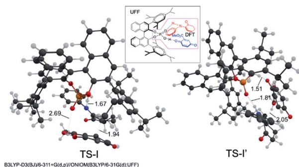
Fig. 4 Optimized geometries and the key bond lengths of TS-I and TS-I' with CPA5.
