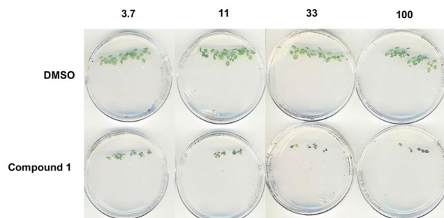
Figure 5. Compound 1 tested against Arabidopsis seedlings at 3.7 \mu\text{M} , 11 \mu\text{M} , 33 \mu\text{M} and 100 \mu\text{M} . Treatment restricted growth and led to purple leaf patches at 11 \mu\text{M} and above compared to the DMSO control.
