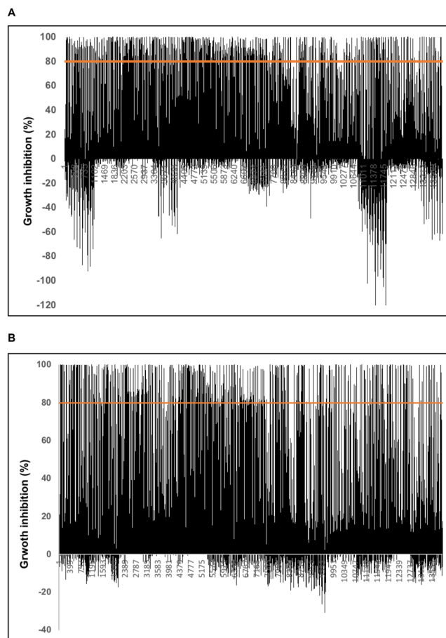
Figure 3. Growth inhibition for compounds (10 \mu\text{M} ) against AtIPCS2 (A) and Aur1p (B) complemented yeast. After eliminating false positives (2.6%), 106 target directed hits were identified, a hit rate of 0.9%.
