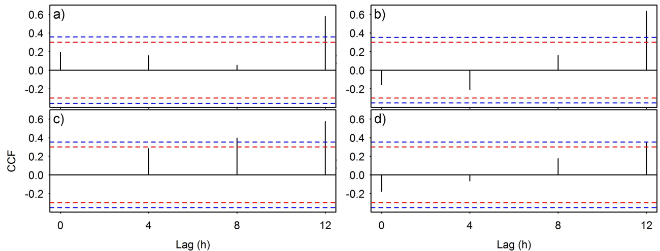
Fig 5. Cross-correlations between animal counts and environmental parameters. Analyses used to assess the presence of temporal lag in the response of animal behavior to environmental fluctuations; a) and b) A. fimbria and flow magnitude in June and July respectively, c) E. stoutii and chlorophyll concentration in December and finally, d) juvenile crabs and oxygen concentration in December. “Cross-Correlation Function, (CCF)” is the measure of the power of the statistic. The dashed blue lines represent a CCF significance for \alpha = 0.05 (critical values: \pm 1.96/\sqrt{n} = \text{approx. } \pm 0.36 in a, and \pm 0.35 in b, c and d, where n is the sample size). The dashed red lines represent a CCF significance for \alpha = 0.1 (accordingly, critical values: \pm 1.65/\sqrt{n} = \text{approx. } \pm 0.3 in all four plates).
