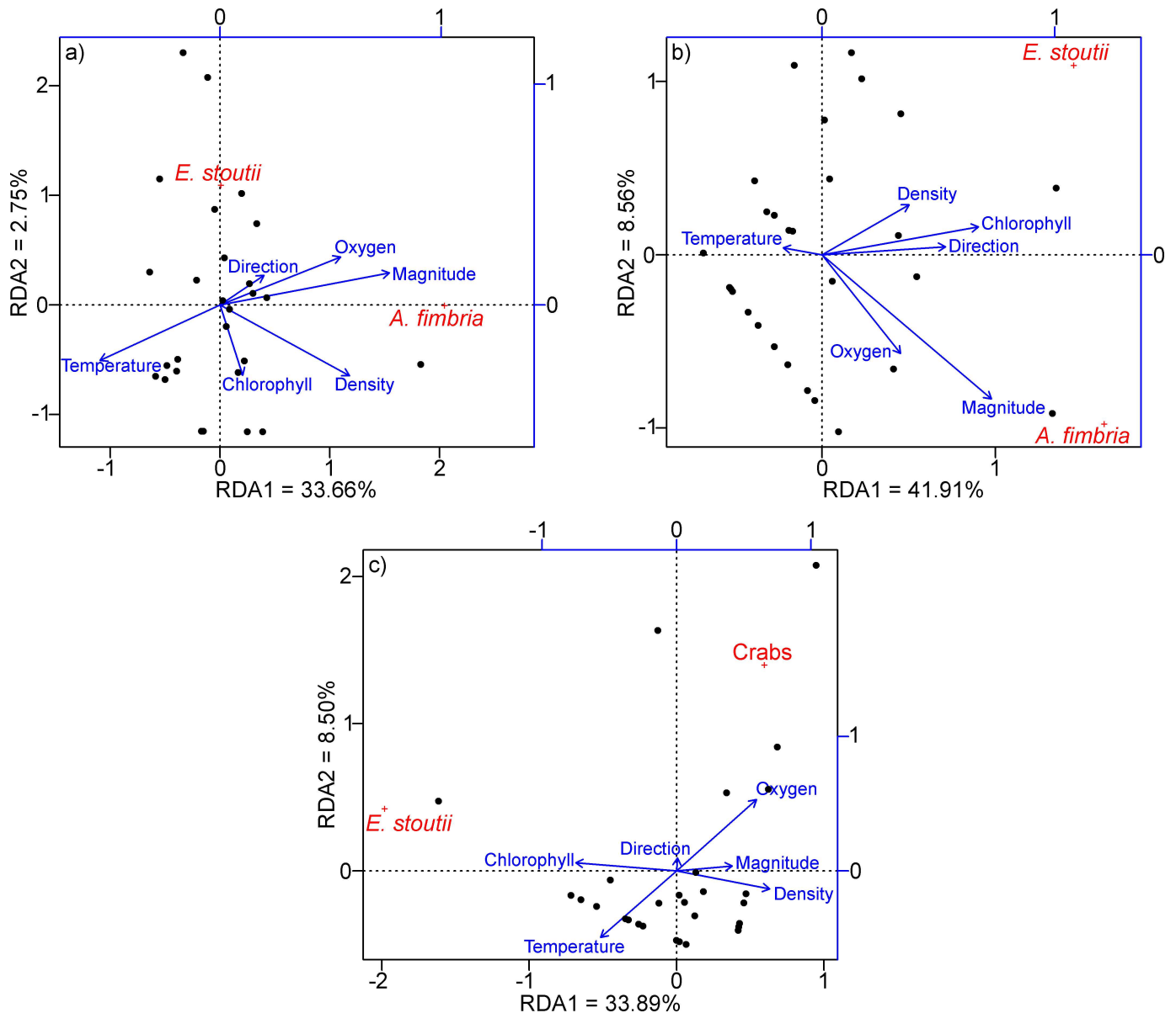
Fig 6. Redundancy Analysis (RDA) of the hydrates benthic community. RDA biplots for each one of the three months of the study period; a) June, b) July and c) December. The direction and length of the blue vectors depicting environmental variables represent positive or negative correlation with the ordination and proportionality of correlation respectively. Their biplot scores are depicted on the blue axes (normalized range -1 to 1). The scores for sites and species are weighted for scaling reasons and depicted on the black axes.
