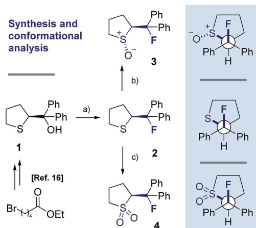
Scheme 1 Synthetic route to the cyclic sulfide 2 , sulfoxide 3 and sulfone 4 from 1 . (a) DAST, \text{Na}_2\text{CO}_3 , \text{CH}_2\text{Cl}_2 , 0\text{ }^\circ\text{C} to rt, 16 h; (b) mCPBA (1.0 eq.), \text{CH}_2\text{Cl}_2 , 0\text{ }^\circ\text{C} to rt, 50 h; (c) mCPBA (3.0 eq.), \text{CH}_2\text{Cl}_2 , 0\text{ }^\circ\text{C} to rt, 17 h.
