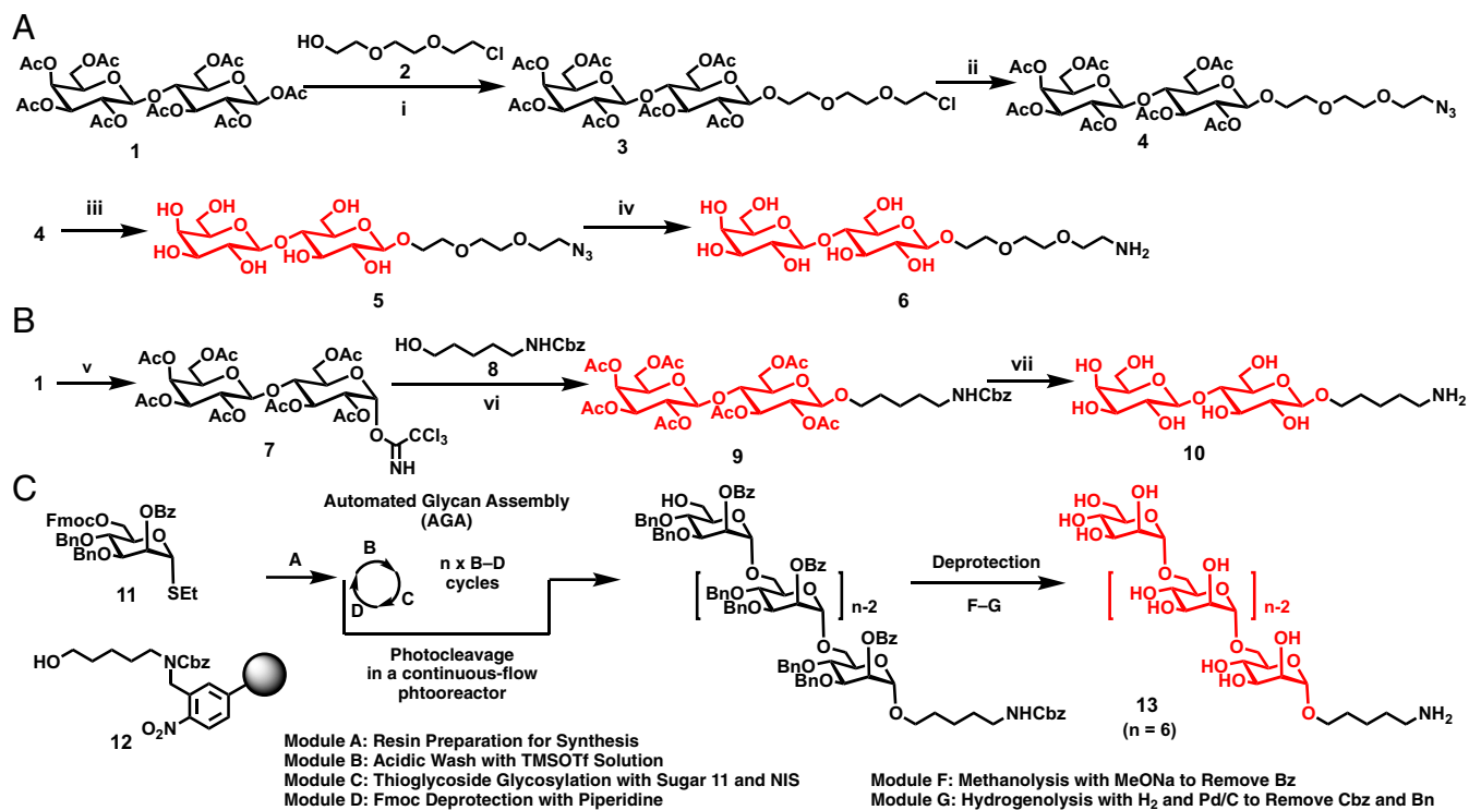
Fig. 1. Synthetic route for preparation of sugars containing triethylene glycol azido and amino linkers ( A ). Synthetic route for sugar containing the hydrophobic N -pentyl amino linkers ( B ). Automated glycan assembly of oligoMan containing N -pentyl amino linkers ( C ). Reagents and conditions: (i) \text{BF}_3 \cdot \text{Et}_2\text{O} , \text{CH}_2\text{Cl}_2 , 0 °C to 23 °C, 15 h, 80%; (ii) \text{NaN}_3 , DMF, 80 °C, 15 h, 74%; (iii) MeONa, methanol, pH = 10, 23 °C, 7 h, 95%; (iv), \text{H}_2 , Pd/C, methanol, 23 °C, 15 h, 95%; (v) \text{H}_2\text{NNH}_2 \cdot \text{HOAc} , DMF, then \text{CCl}_3\text{CN} , DBU, \text{CH}_2\text{Cl}_2 , 79%; (vi) TMSOTf, \text{CH}_2\text{Cl}_2 , 39%; (vii) MeONa, methanol, then \text{H}_2 , Pd/C, 82%.
