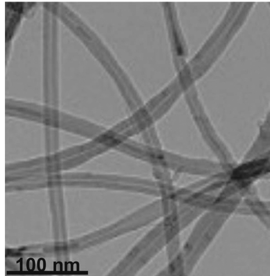
Fig. 2. Transmission-electron-microscope micrograph of DNA nanotubes. The nanotubes have micron lengths with nanoscale widths. The micrograph was obtained with Philips EM028 transmission electron microscope equipped with field-emission gun.
