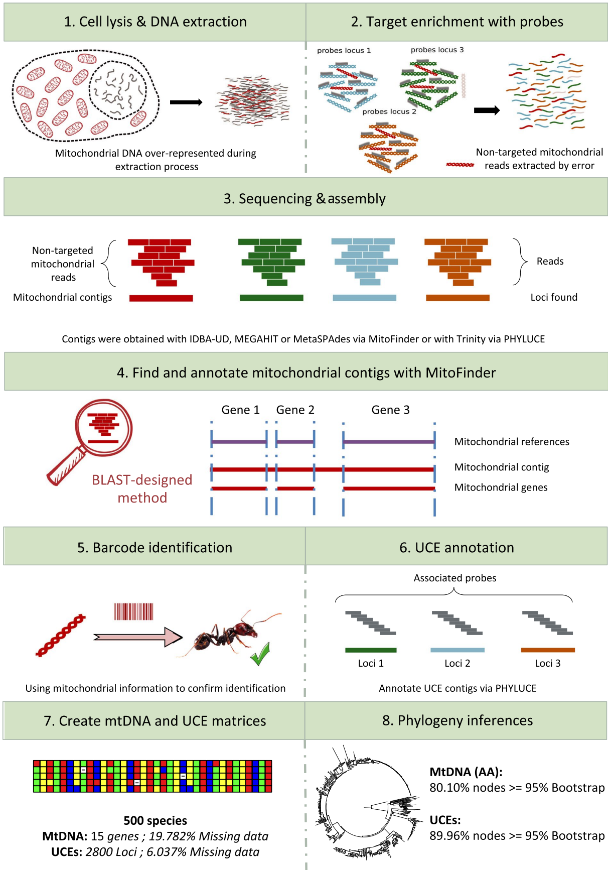
FIGURE 1 Conceptualization of the pipeline used to assemble and extract UCE and mitochondrial signal from ultraconserved element sequencing data [Colour figure can be viewed at wileyonlinelibrary.com ]
