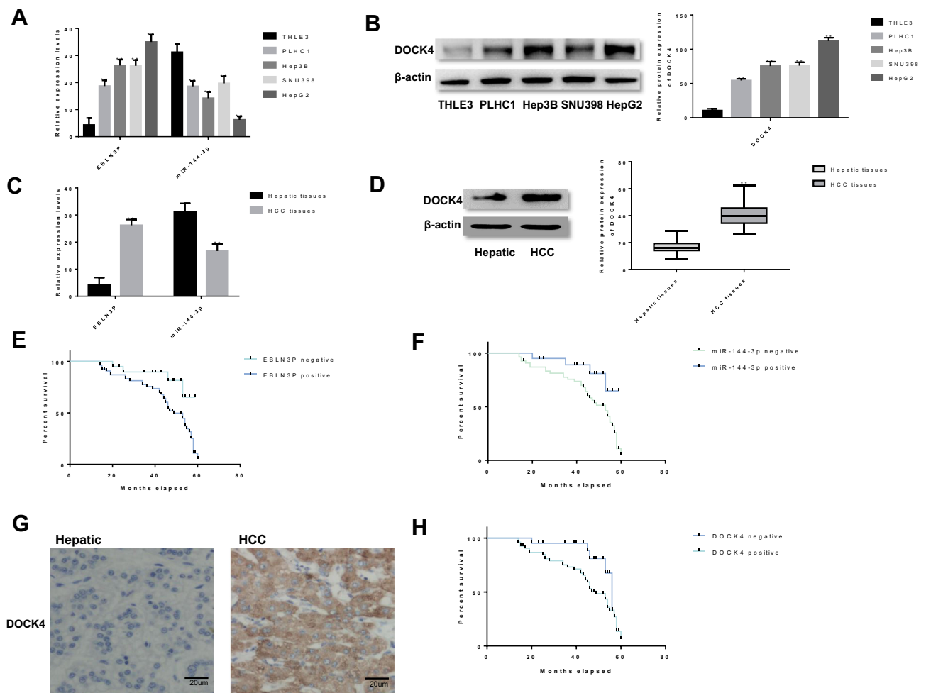
Figure 4 EBLN3P and DOCK4 were upregulated, while miR-144-3p was downregulated in liver cancer tissues and cell lines. (A) The expression levels of EBLN3P and miR-144-3p in liver cancer cell lines (PLHC1, Hep3B, SNU398 and HepG2) and the hepatocyte cell line (THLE3) were tested by RTq-PCR. (B) The Western blotting results showed that DOCK4 was expressed at a higher level in four liver cancer cell lines (PLHC1, Hep3B, SNU398 and HepG2) than in the normal human hepatic astrocyte cell line (THLE3). (C) The expression patterns of EBLN3P and miR-144-3p were measured in liver cancer samples and normal tissue via RTq-PCR. (D) The expression patterns of DOCK4 were measured in liver cancer samples and normal tissue via Western blotting. (E) The association between EBLN3P expression and the prognosis of patients with liver cancer was explored. (F) The association between miR-144-3p expression and the prognosis of patients with liver cancer was explored. (G) The expression patterns of DOCK4 were measured in liver cancer samples and normal tissue via immunohistochemistry. (H) The association between DOCK4 expression and the prognosis of patients with liver cancer was explored. The data are shown as the mean \pm SD. ** P < 0.01 .
