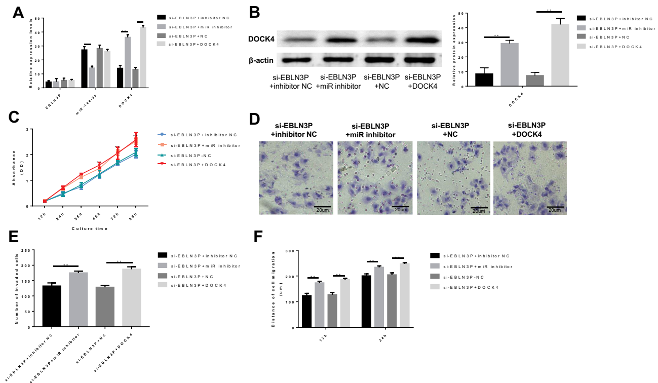
Figure 3 EBLN3P regulates liver cancer cells via the miR-144-3p/DOCK4 pathway. High mRNA (A) and protein (B) expression level of DOCK4 was achieved by transfecting cells with pcDNA3.1- DOCK4 or miR-144-3p inhibitor. Knockdown of EBLN3P markedly reduced cell proliferation (C), invasion (D and E) and migration (F). However, compared to transfection with sh- EBLN3P alone, co-transfection with sh- EBLN3P and miR-144-3p inhibitor or DOCK4 significantly increased cell proliferation (C), invasion (D and E) and migration (F). The data are shown as the mean \pm SD. ** P < 0.01 .
