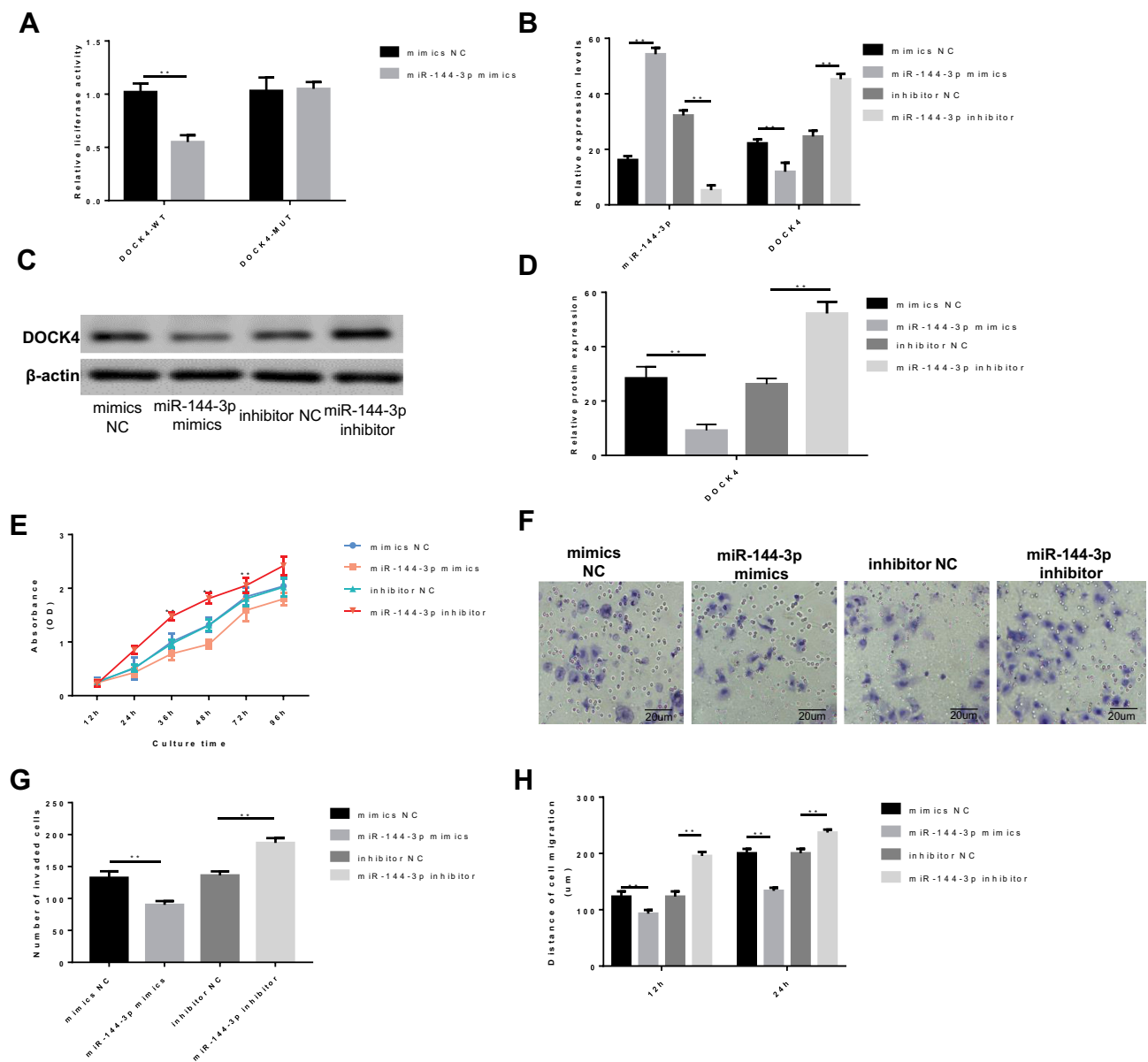
Figure 2 miR-144-3p inhibits the proliferation, migration and invasion of liver cancer cells by downregulating DOCK4 . (A) The miR-144-3p mimics and luciferase reporter plasmids containing wild-type or mutant DOCK4 3'-UTR were cotransfected into HepG2 cells. The dual luciferase reporter gene assay was performed to verify the direct binding association between miR-144-3p and DOCK4 . (B) HepG2 cells were transfected with NC mimics, miR-144-3p mimics, NC inhibitor, or miR-144-3p inhibitor, and then, reverse transcription-quantitative PCR was conducted to evaluate the relative expression levels of miR-144-3p and DOCK4 . (C) Western blotting validated that the overexpression of miR-144-3p significantly decreased DOCK4 expression. (D) Corresponding analysis of DOCK4 expression. (E) Cell proliferation was tested by the Cell Counting Kit-8 assay. (F) Cell invasion was detected by the Transwell assay. (G) The number of invaded cells. (H) Cell migration was detected by the wound healing assay. The data are shown as the mean \pm SD. ** P < 0.01 .
