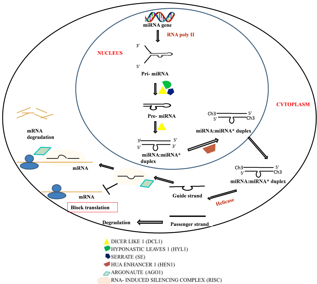
Figure 1. Mechanism of miRNA biogenesis and gene silencing. The miRNA biogenesis commences with the transcription of miRNA genes into pri-miRNA by RNA polymerase II, which is further subjected to primary and secondary processing via the enzyme complex of DCL-1, SE, and HYL1 leading to the generation of pre-miRNA and an miRNA/miRNA* duplex, respectively. Further the HEN1-mediated methylation at the 3'-OH end leads to the export of the duplex to the cytoplasm. In the cytoplasm, the passenger RNA strand is degraded and the guide strand from the miRNA-inducing silencing complex (miRISC) directs the degradation or translation inhibition of the target mRNA.
