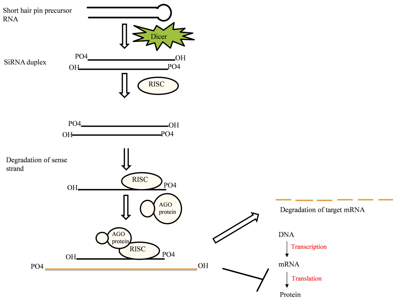
Figure 2. siRNA biogenesis and gene silencing. Here the action of Dicer or the Dicer-like enzyme on the precursor RNA results in an siRNA duplex with overhangs at 3'-OH ends. Further, the antisense strand from siRNA induces the silencing complex by associating with the RISC protein. Thereafter, incorporation of AGO and other effector proteins with siRISC facilitate the gene silencing through degradation of the target mRNA or translation inhibition.
