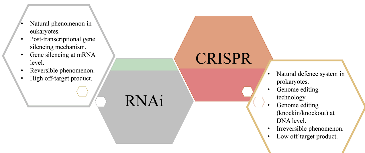
Figure 4. RNA interference vs. the CRISPR/Cas9 system.
