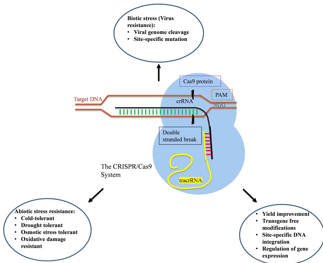
Figure 3. Applications of the CRISPR/Cas9 system in crop improvement. Here, the omission of undesirable traits and the adjunction of purposeful traits occurs through highly specific targeted genome modification.
