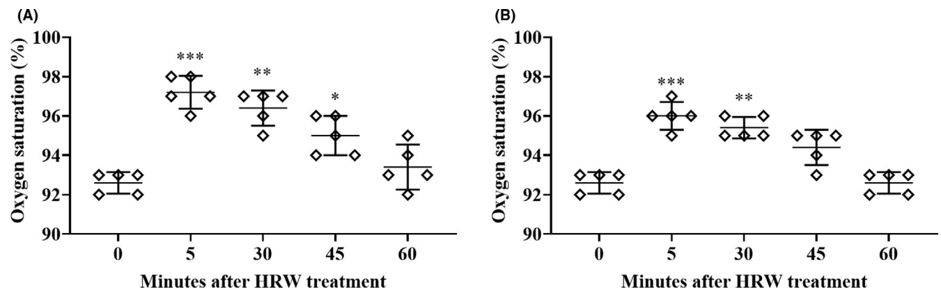
FIGURE 1 Mean oxygen saturation following five-day treatment with HRW. (A) treatment with three H 2 -producing tablets in the morning; (B) treatment with two H 2 -producing tablets in the evening. Hydrogen-producing tablets were dissolved in 200 mL of water each for a total daily intake of 1L of HRW. The results are presented graphically as mean \pm SD with individual values for each daily measurement. * p < 0.05 , ** p < 0.01 , *** p < 0.001 as compared to 0 (before treatment). Statistical differences were analyzed using repeated measure one-way analysis of variance (ANOVA), followed by Tukey's Multiple Comparison Test using GraphPad Prism Software, ver. 8.0.2. (GraphPad Software).
