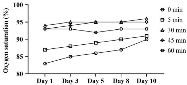
FIGURE 2 Time course of oxygen saturation after daily HRW treatment followed by exercise. The baseline SpO 2 measurements (0 min) were performed just prior to HRW treatment
