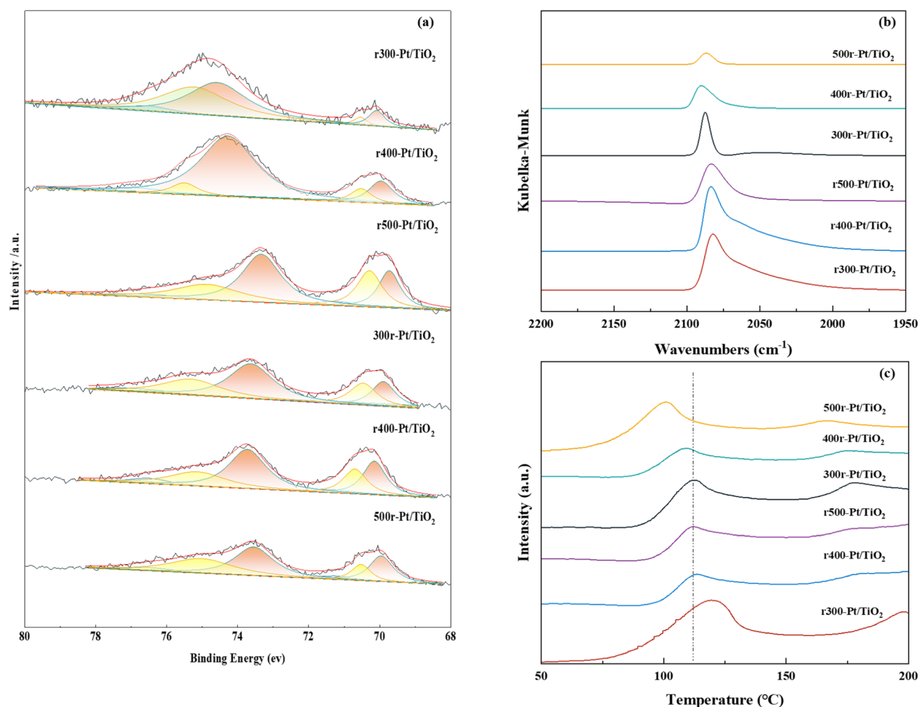
Fig. 4 Pt 4f XPS spectra (a), in situ CO-DRIFT spectra (b), H 2 -TPD profiles (c) of the prepared sample.
