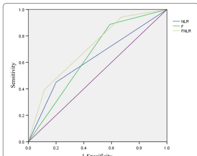
Fig. 1 ROC curve for fibrinogen, NLR and F-NLR in OSCC patients. Fibrinogen, NLR, and F-NLR were the test variables, and CSS was the state variable. The areas under the curve are 0.649, 0.625 and 0.713, respectively. ROC receiver operating characteristic, F-NLR combined fibrinogen and NLR score, NLR neutrophil-to-lymphocyte ratio, CSS cancer-specific survival, OSCC oral squamous cell carcinoma, F fibrinogen
