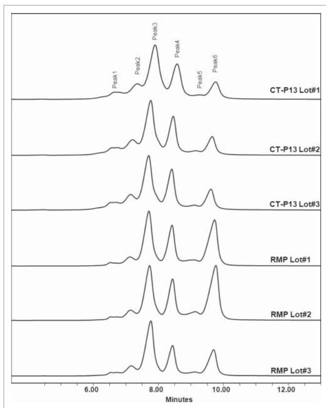
Figure 9. Comparison of charge profiles between RMP and CT-P13 analyzed by Cation Exchange Chromatography.
