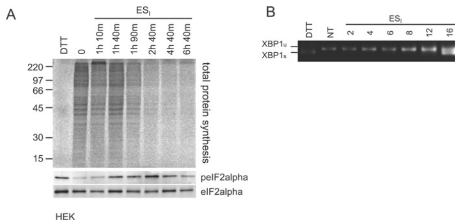
Figure S3 ES 1 activates the UPR in HEK cells
