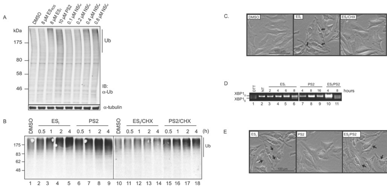
Figure S4 Relationship between ES 1 and the UPS
