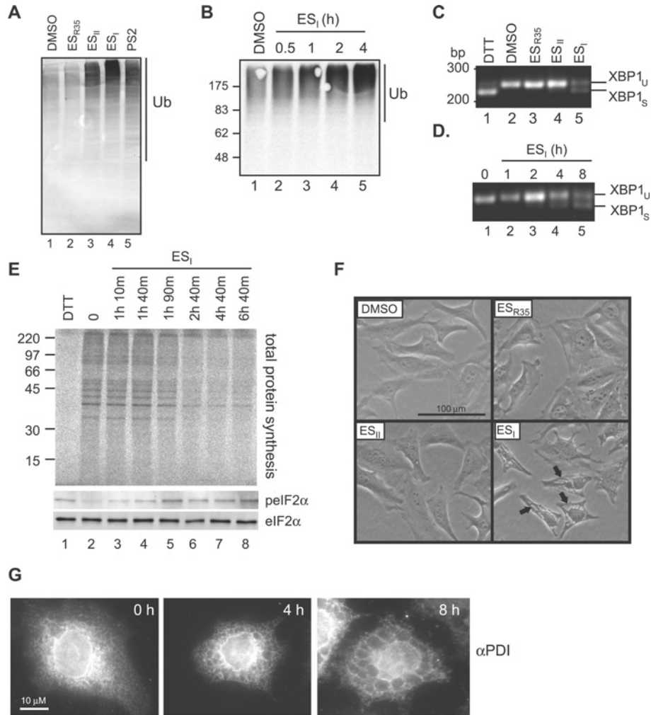
Figure 1 Cellular effects of ES compounds
