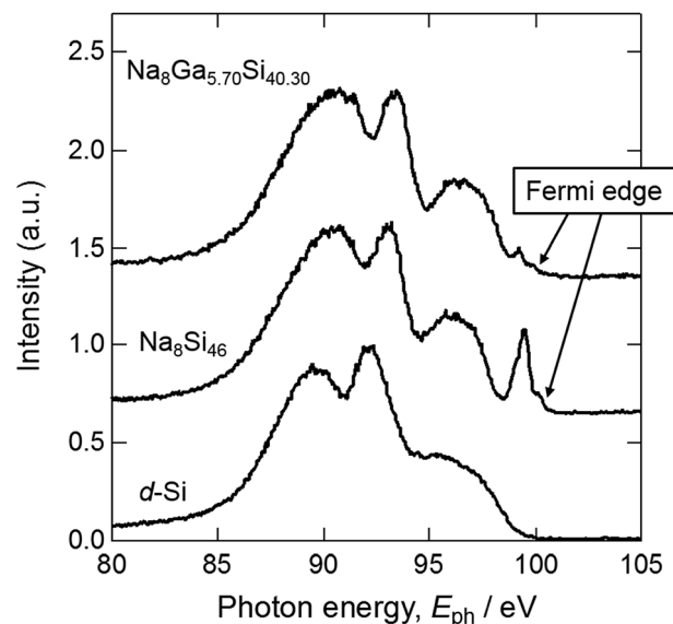
Fig. 6 Si L_{2,3} SXE spectra of \text{Na}_8\text{Ga}_{5.70}\text{Si}_{40.30} , \text{Na}_8\text{Si}_{46} , and d-Si.
