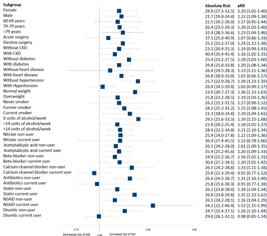
Figure 3 Forest plot (subgroup analyses). Current use of ACE inhibitors and/or angiotensin receptor blockers and the risk of acute kidney injury within 7 days after colorectal cancer surgery across subgroups of demographics and comorbidities. Underweight, <18.5 kg/m 2 ; normal weight, 18.5–25 kg/m 2 ; overweight, >25 kg/m 2 . AKI, acute kidney injury; aRR, adjusted relative risk; CKD, chronic kidney disease; NSAID, non-steroidal anti-inflammatory drug.
