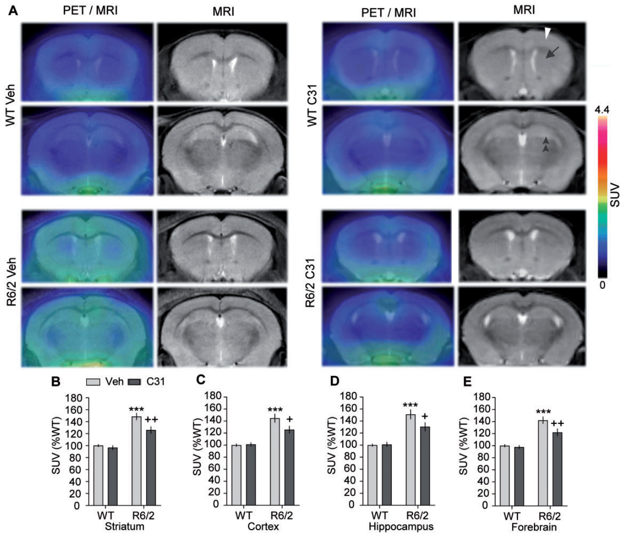
Figure 3. [ ^{18}\text{F} ]PBR06-PET detects reduced TSPO levels in R6/2 mice treated with LM11A-31. (A) Representative PET and MR images of coronal sections of the striatum (black arrow), cortex (white arrowhead) and hippocampus (two black arrowheads) of WT and R6/2 mice with and without LM11A-31 (C31) treatment. PET/MRI overlay is in the left columns and MRI alone is in the right columns. (B–E) Quantification of [ ^{18}\text{F} ]PBR06 uptake in striatum (B), cortex (C), hippocampus (D), and forebrain (E) of WT-Veh ( n = 14 ), WT-C31 ( n = 8 ), R6/2-Veh ( n = 10 ) and R6/2-C31 ( n = 11 ) groups. Results are expressed as standardized uptake value (SUV) mean \pm s.e.m. and normalized to the PET signal of the WT-Veh within each group of four mice imaged at the same time to minimize variability between imaging sessions. Statistical significance was determined with an ANOVA and Fisher's LSD. *** P < 0.0001 versus WT-Veh; + P < 0.01 and ++ P < 0.01 versus R6/2-Veh.
