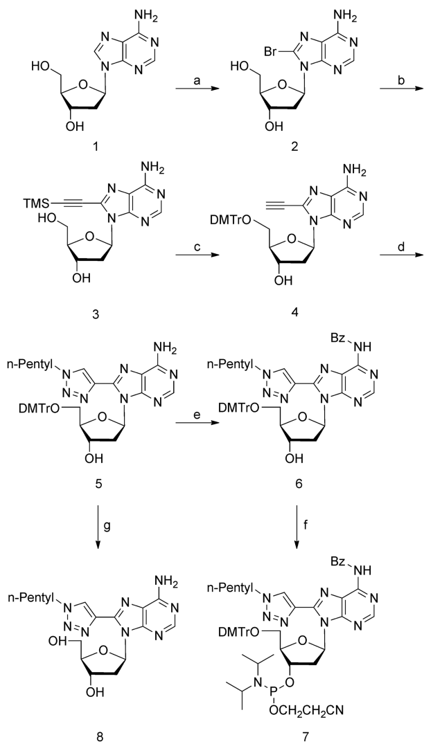
Scheme 1. (a) \text{Br}_2/\text{NaOAc} -buffer, r.t., overnight, 81%. (b) \text{Pd}(\text{PPh}_3)_4 (4 mol%), \text{CuI} (8 mol%), TMS-acetylene, Amberlite IRA-67, THF, 40^\circ\text{C} , 2 h, 91%. (c) (i) DMTrCl, pyridine, overnight, r.t.; (ii) \text{NH}_3 (25% aq.), 2 h 65%. (d) (i) Pentylbromide, \text{NaN}_3 , water, 140^\circ\text{C} , 1 h; (ii) \text{CuI} , ethyl acetate, 14 h, r.t., 76%. (e) (i) TMSCl, pyridine, 2 h; (ii) \text{BzCl} , 3 h; (iii) Water, 15 min then \text{NH}_3 (aq.), 30 min, 68%. (f) DIPEA (0.11 ml, 0.64 mmol), 2-Cyanoethyl- N,N -diisopropylchlorophosphoramidite, DCM, 1 h, 91%. (g) Acetic acid, 30 min, 34%.
