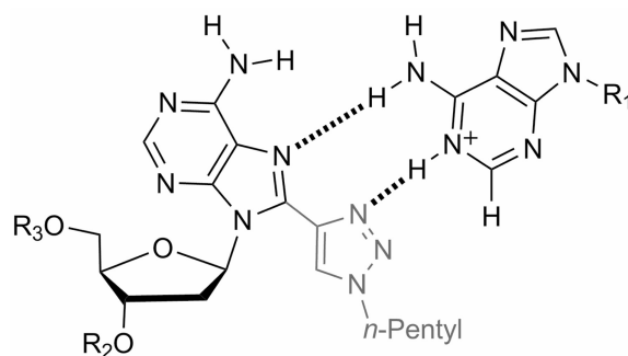
Figure 6. Putative stabilized A^T .A base pair. Only the sugar attached to A^T is shown and its triazole and pentyl chain are coloured grey. R_1 , R_2 and R_3 represent the rest of the DNA structure.
