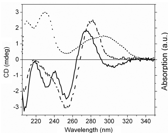
Figure 5. CD spectra of the modified GG -duplex (solid line) and of the corresponding natural duplex (dashed line). The difference in absorption spectra of A^T and A (dotted line) was obtained by subtracting the absorption spectra of equimolar solutions of the natural GG -duplex from the modified GG -duplex. Spectra were recorded in phosphate buffer (500 mM Na^+ , pH 7.5) at 25°C at a duplex concentration of 2.5 \mu M.
