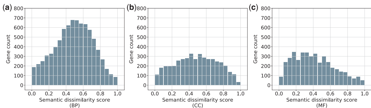
Fig. 4. Distributions of semantic dissimilarity scores of MIGs that have functionally divergent isoforms. The range of semantic dissimilarity score [0, 1] is equally divided into 20 bins. For each bin, we count how many MIGs have semantic dissimilarity scores in this range. The three GO branches are considered separately
