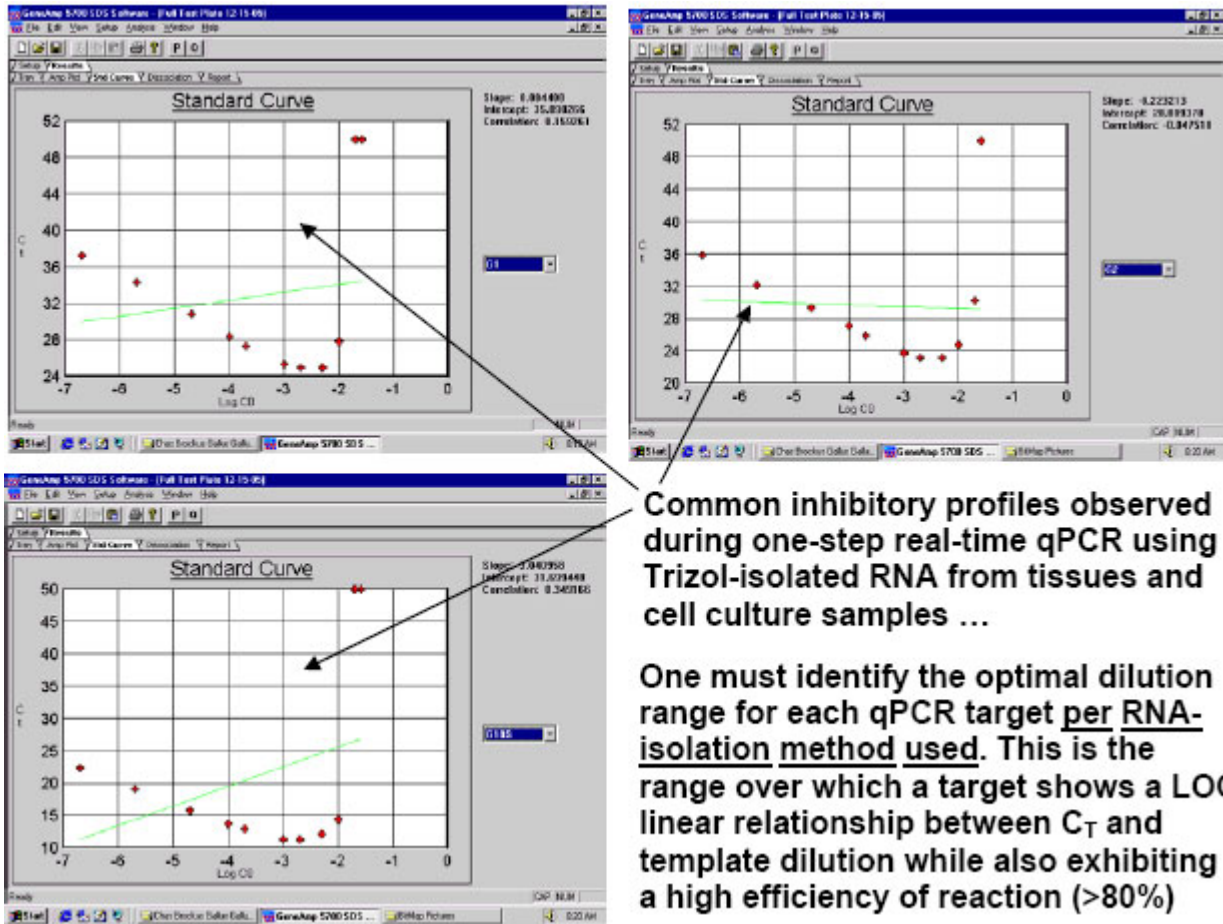
Fig. 5: Demonstration of typical inhibitory qPCR profiles exhibited on qPCR Test Plates by the more concentrated RNA samples (on the right hand side of each graph) in a progressive dilution series. Targets here were Gallus gallus Gallinacin 1, Gallinacin 2 and Gallus gallus 18S ribosomal RNA (the single housekeeper). Stock I here was an equivolumetric mixture of the 26 total tissue RNA samples used in this study: just after their isolation by Trizol method, each RNA pellet was resolubilized in 150 \mu l of 0.1 mM EDTA pH 6.75, warmed to 65 ^{\circ} C for 5 minutes, and their 260 nm and 260 nm /280 nm measurements at 1:50 were taken. 70 \mu l of each resolubilized RNA was then Turbo-DNase treated [70 \mu l RNA isolate + 10 \mu l 10X Turbo DNase Buffer + 20 \mu l Turbo DNase enzyme (40 Units); and finally 10 \mu l Inactivation Reagent] and 80 \mu l of each was then diluted 1:10 with nuclease-free water. Subsequently, 50 \mu l of each of these 1:10 RNA isolates was mixed together into a single tube attaining a final volume of 1,300 \mu l. This was the Stock I RNA solution from which all standards and inter-plate calibrators were prepared. It was also the mixture which served as the source of the serially-diluted template samples for the Test Plate which we ran early on to identify the best RNA dilution ranges for each of the 3 targets. All calculations for this study were quickly performed by the FF2-6-001 qPCR set-up tool.
