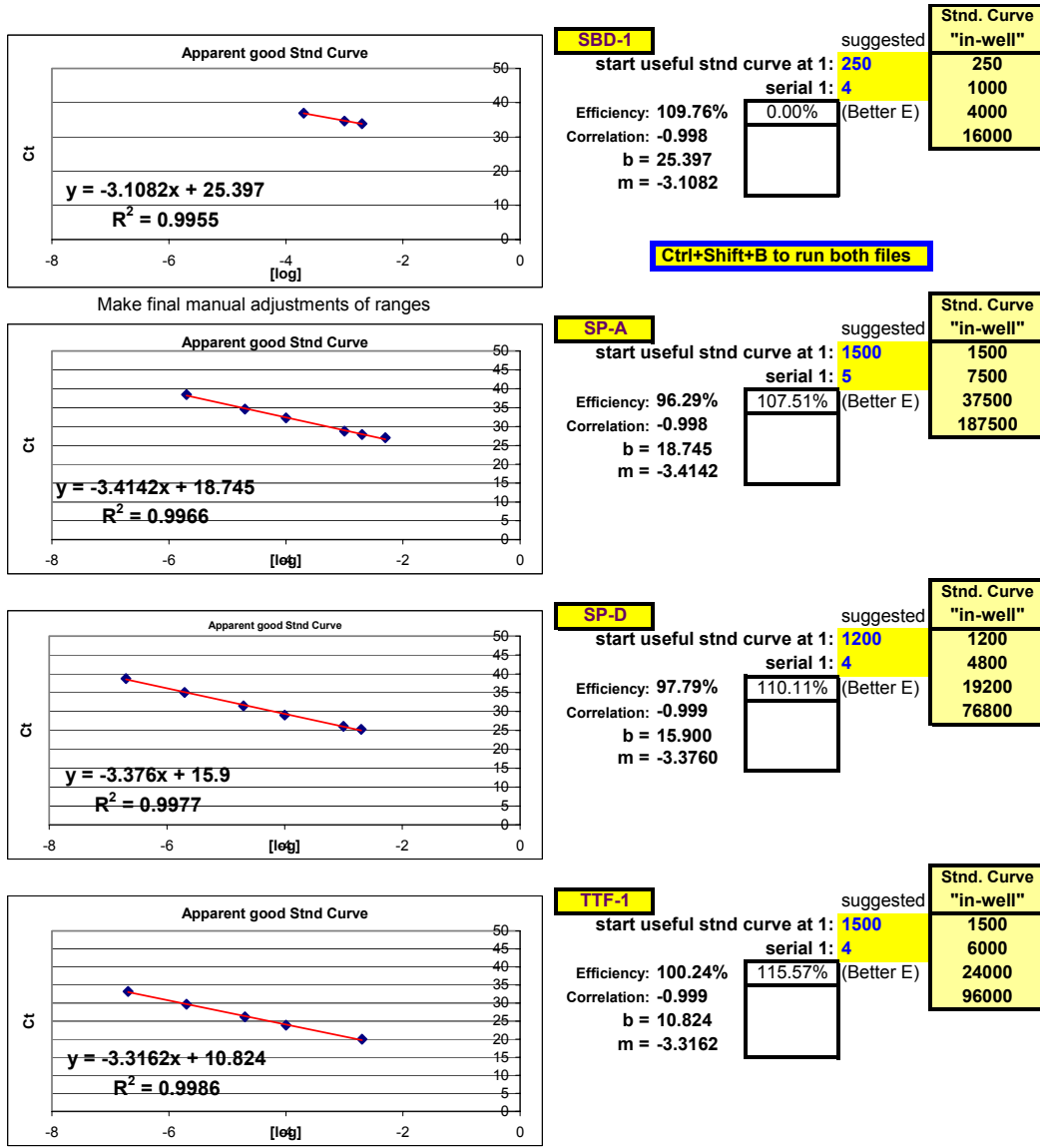
Fig. 25: Optimal ranges identified for all targets using the FF2-6-001 qPCR set-up tool TestPlateResultsAnalysis2006.xls file (which is connected by Visual Basic macros and equations to its "twin" file, TestPlateResultsAnalysis2006b.xls, which is used to fine-tune the parameters revealed by this file). Efficiencies and slopes for each target are calculated from Test Plate C T values for each qPCR target as the user manually selects different points on each graph in effort to ascertain the optimal RNA dilution ranges for each target.
