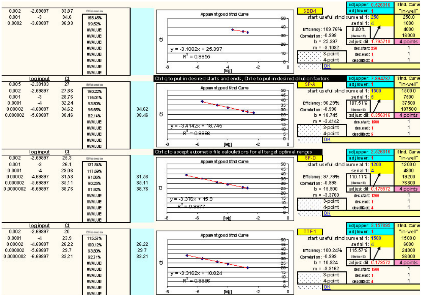
Fig. 30: Portion of the FF2-6-001 qPCR set-up tool TestPlateResultsAnalysis2006b file which allows the user to fine-tune the parameters already established by "twin" file TestPlateResultsAnalysis2006. In this file, the user manually adjusts standard curve dilution factors, standard curve start and end points (or chooses to accept file default calculations for those parameters), and activates pre-programmed macros to quickly hone in on the final optimal RNA dilution range to be used for each target – all of which exhibit LOG-linear behavior, lack of qPCR inhibition and high amplification reaction efficiencies; all based on Test Plate C_T analyses.
