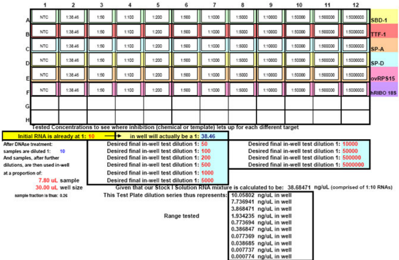
Fig. 28: Depiction of a six-target Test Plate profile. After running the plate, the C T results are fed into FF2-6-001 qPCR set-up tool TestPlateResultsAnalysis2006.xls and TestPlateResultsAnalysis2006b.xls files to identify the dilution ranges for each target which allow each target to amplify with desirable efficiency undaunted by inhibition of any kind. A slope of -3.3219 or (-1/LOG 10 2) represents 100% efficiency when C T values are plotted against the LOG 10 of template input dilution factors. In our approach, C T values are generated from a standard set of eleven serial progressive dilutions of Stock I resulting in 'dilution,' 'calibration' or 'standard' curves for each target. Analyzing Test Plate C T values allows the investigator to identify the RNA sample dilution ranges for each target within which each target remains uninfluenced by inhibitory phenomena and is allowed to achieve acceptable amplification reaction efficiency somewhere along the RNA dilution profile. Dilution curve slopes ranging from -4.11 to -3.01 (or a reaction efficiency range of 75 to 115%, respectively) are considered to be acceptable in most real-time qPCR assays. The Test Plate-attained slopes for the above six targets are shown in Figure 27.
