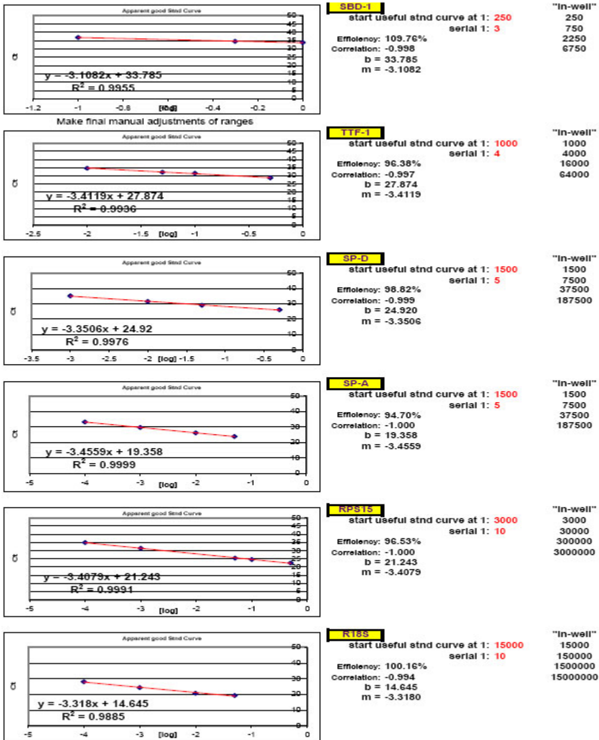
Fig. 27: Additional example of optimal ranges identified for a different group of qPCR targets. Again, reaction efficiencies (or 'efficacies') and slopes were calculated from Test Plate C T values for each qPCR target dilution to ascertain the optimal RNA dilution ranges for each of the targets. (Early prototype versions of FF2-6-001 qPCR set-up tool TestPlateResultsAnalysis2006.xls and TestPlateResultsAnalysis2006b.xls files were used to make the determinations shown here).
