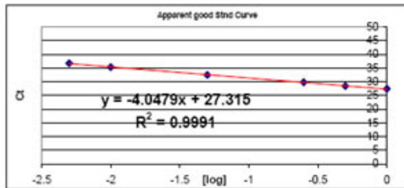
Fig. 3: (Marligen) column-isolated/purified RNA exhibits a lower threshold of qPCR inhibition. Inhibition Types 1, 2 and 3 are presumably demonstrated with the first dilution point shown here. Marligen Rapid Total RNA Purification System RNA isolation from equine dendritic cells: inhibitory phenomena are not apparent beyond a dilution of 1:50 using RNA isolated by this method. Rare qPCR targets often exhibit lower amplification efficiencies.
