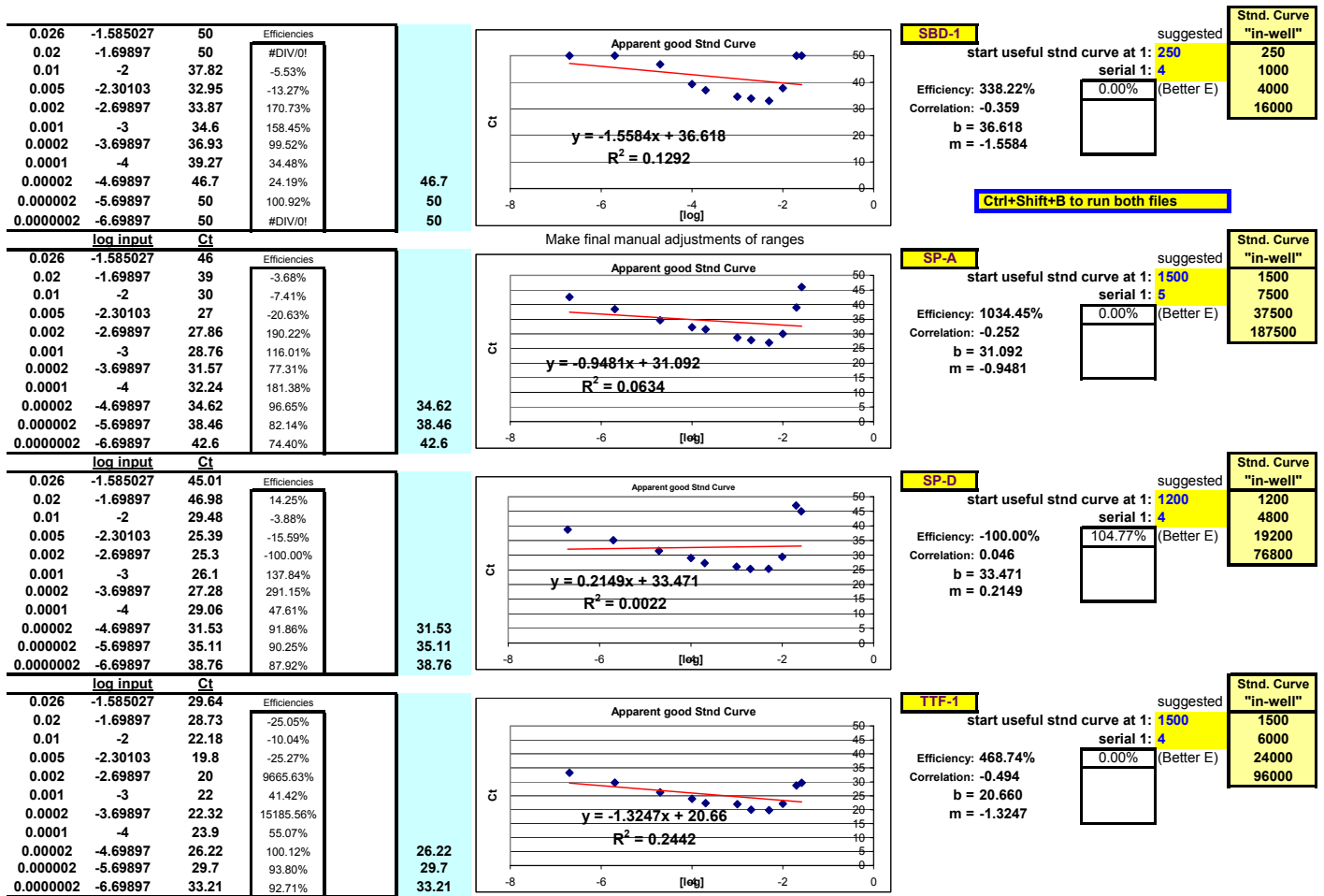
Fig. 24: A portion of FF2-6-001 qPCR set-up tool TestPlateResultsAnalysis2006.xls file just after Test Plate C T values have been entered and preliminary macros have been run. Notice how the regions of qPCR inhibition are clearly exposed for each qPCR target at the right hand side of each target's dilution profile (LOG 10 of Stock I dilution vs. C T ) graph. The most concentrated RNA samples in each case are the samples which exhibit the most qPCR inhibitory phenomena.
