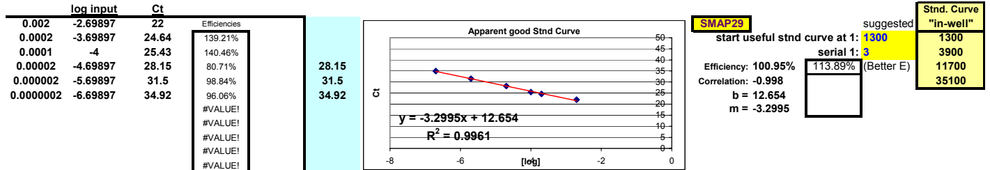
Fig. 26: Close up of a region of the FF2-6-001 qPCR set-up tool TestPlateAnalysis2006.xls file which is used to detect qPCR inhibition, dial in a target's optimal RNA dilution range, and find the Stock I RNA dilution range which yields the highest efficiency reaction for each qPCR target. Here, qPCR target SMAP29 has been assessed.
