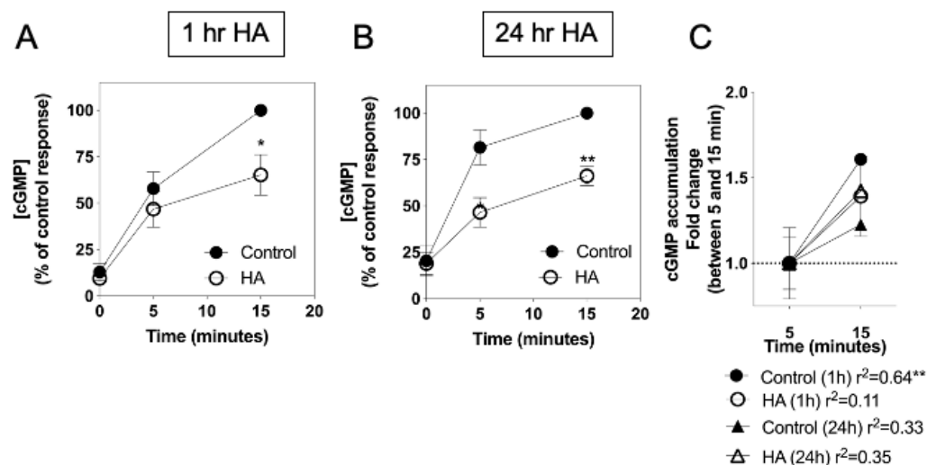
Figure 3. Effects of hyperammonaemia on CNP-stimulated cGMP accumulation in rat C6 glioma cells. Cells were initially treated in media containing 1% ( v/v ) FCS and 0 or 10 mM \text{NH}_4\text{Cl} (HA) for either (A) 1 h or (B) 24 h, prior to subsequent stimulation with 100 nM CNP in the presence of 1 mM IBMX for up to 15 min. The data shown are means \pm SEM of five to seven independent experiments, each performed in triplicate and are expressed as the percentage of the control; * p < 0.05 , ** p < 0.01 , significantly different from control response to CNP. (C) Linear accumulation of cGMP between 5 and 15 min of CNP stimulation. Data shown are normalized to cGMP accumulation after 5 min, expressed as means \pm SEM of five to seven independent experiments. ** p < 0.01 , significantly deviates from zero.
