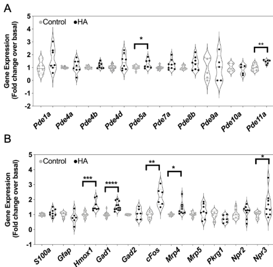
Figure 6. Effects of hyperammonaemia on cGMP-associated, and astrocyte-enriched gene expression in rat C6 glioma cells. Cells were initially treated in media containing 1% ( v/v ) FCS and 0 or 10 mM \text{NH}_4\text{Cl} (HA) for 48 h, prior to extracting total RNA. Multiplex RT-qPCR assays were performed on RNA extracted from C6 cells to detect (A) transcripts encoding phosphodiesterase enzymes, (B) other cGMP-associated genes and astrocyte-enriched transcripts. The data shown are the medians (with 5 to 95% confidence intervals) of relative gene expression, normalized to Actb and expressed as fold change over basal, from 4 to 12 individual RNA extractions. * p < 0.05 , ** p < 0.01 , *** p < 0.001 , **** p < 0.0001 , significantly different from control.
