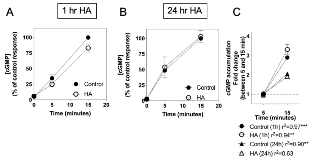
Figure 4. Effects of hyperammonaemia on SNP-stimulated cGMP accumulation in rat C6 glioma cells. Cells were initially treated in media containing 1% ( v/v ) FCS and 0 or 10 mM \text{NH}_4\text{Cl} (HA) for either (A) 1 h or (B) 24 h, prior to subsequent stimulation with 1 mM SNP in the presence of 1 mM IBMX for up to 15 min. The data shown are means \pm SEM of three independent experiments, each performed in triplicate and are expressed as the percentage of the control response to SNP. (C) Linear accumulation of cGMP between 5 and 15 min of SNP stimulation. Data shown are normalized to cGMP accumulation after 5 min, expressed as means \pm SEM of three independent experiments. *** p < 0.001 , ** p < 0.01 , significantly deviates from zero.
