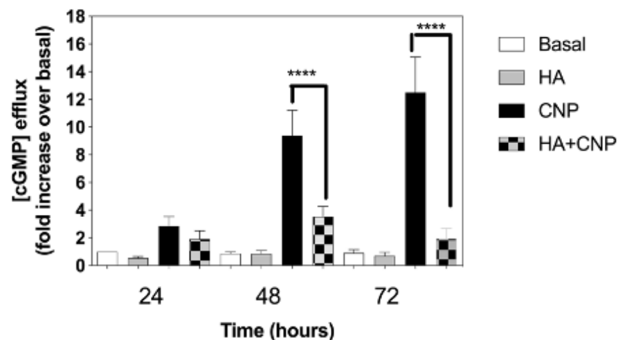
Figure 5. Effects of hyperammonaemia on CNP-stimulated cGMP efflux rat C6 glioma cells. C6 cells were treated in media containing 1% ( v/v ) FCS and either 0 or 10 mM \text{NH}_4\text{Cl} , (HA) in the absence or presence of 100 nM CNP, for up to 72 h. Spent media were collected at the indicated time points and analysed for cGMP content. Data shown are means \pm SEM of 6 to 8 independent experiments, each performed in triplicate, and normalized to basal at each time point. **** p < 0.0001 , significantly different to control response to CNP.
