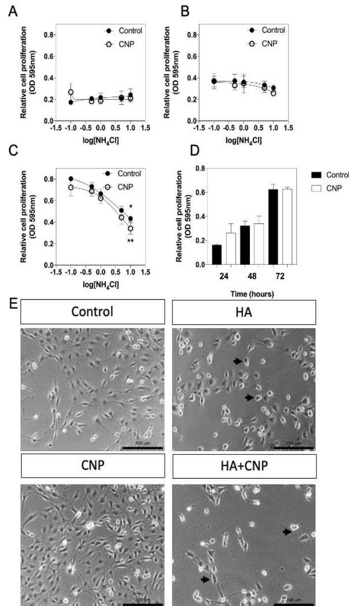
Figure 2. Effects of hyperammonaemia and CNP on cell proliferation and morphology in rat C6 glioma cells. C6 cells were treated with the indicated concentrations of \text{NH}_4\text{Cl} (log mM) (as an \text{NH}_3 donor) in the absence or presence of 100 nM CNP for (A) 24 h, (B) 48 h or (C) 72 h, before being fixed in paraformaldehyde, and stained for crystal violet assay. The data shown are means \pm SEM pooled from 3 independent experiments, each performed with 8 replicates. * p < 0.05 , ** p < 0.01 , significantly different from untreated cells. (D) Cell viability in C6 cells in the presence of 0 or 100 nM CNP over 72 h. The data shown are means \pm SEM pooled from 3 independent experiments, each performed with 8 replicates. (E) Representative microscopy images of C6 cells treated for 72 h with 0 (control) or 10 mM \text{NH}_4\text{Cl} (HA), in the presence of 100 nM CNP alone (CNP) or in combination (HA+CNP). Arrow heads indicated rounded cells.
