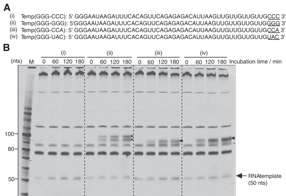
Figure 2 Primer-independent RNA synthesis on RNA templates with NV3D Pol . (A) The sequence of RNA templates. (B) NV3D Pol (5 pmol) was incubated with (i) Temp(GGG-CCC), (ii) Temp(GGG-GGG), (iii) Temp(GGG-CCA) or (iv) Temp(GGG-UAC) (5 pmol each), and sampled at 0, 60, 120, 180 min respectively (reaction volume = 20 \mu L). Each reaction products were separated on an 8 M urea denaturing 10% PAGE, and imaged with Fx imager after SYBRgreenII staining. M; 10 bp DNA step ladder marker (Promega). Black arrow indicates the mobility of each RNA templates (50 nts). For bands indicated by asterisk and short arrows, see text. Other constant bands were from components of cell-free translation system.
