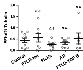
FIGURE 5. EFhd2 protein levels in the frontal cortex are reduced in total homogenates from patients with dementia but not in synaptoneurosomes. (A) Western blots showing EFhd2 protein levels in human frontal cortex tissue extracts from nondemented controls and individuals with Alzheimer disease (AD), frontotemporal lobar degeneration (FTLD)-tau (FTLD-tau), Pick disease, or FTLT-TDP Type B (FTLD-TDP). Beta-actin was used as a loading control for homogenates and nonsynaptic fractions; PSD-95 was used as a loading control for synaptoneurosomes fractions. (B) Quantification of EFhd2 protein bands by densitometry. Error bars = SEM. Homogenate: 1-way ANOVA, p = 0.0301 ; * p < 0.05 compared with control by using Dunnett post hoc test. Synaptoneurosomes: 1-way ANOVA, p = 0.1108 . Nonsynaptic: 1-way ANOVA, p = 0.4848 .
