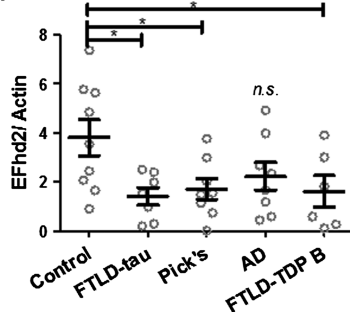
FIGURE 5. EFhd2 protein levels in the frontal cortex are reduced in total homogenates from patients with dementia but not in synaptoneurosomes. (A) Western blots showing EFhd2 protein levels in human frontal cortex tissue extracts from nondemented controls and individuals with Alzheimer disease (AD), frontotemporal lobar degeneration (FTLD)-tau (FTLD-tau), Pick disease, or FTLT-TDP Type B (FTLD-TDP). Beta-actin was used as a loading control for homogenates and nonsynaptic fractions; PSD-95 was used as a loading control for synaptoneurosomes fractions. (B) Quantification of EFhd2 protein bands by densitometry. Error bars = SEM. Homogenate: 1-way ANOVA, p = 0.0301 ; * p < 0.05 compared with control by using Dunnett post hoc test. Synaptoneurosomes: 1-way ANOVA, p = 0.1108 . Nonsynaptic: 1-way ANOVA, p = 0.4848 .
