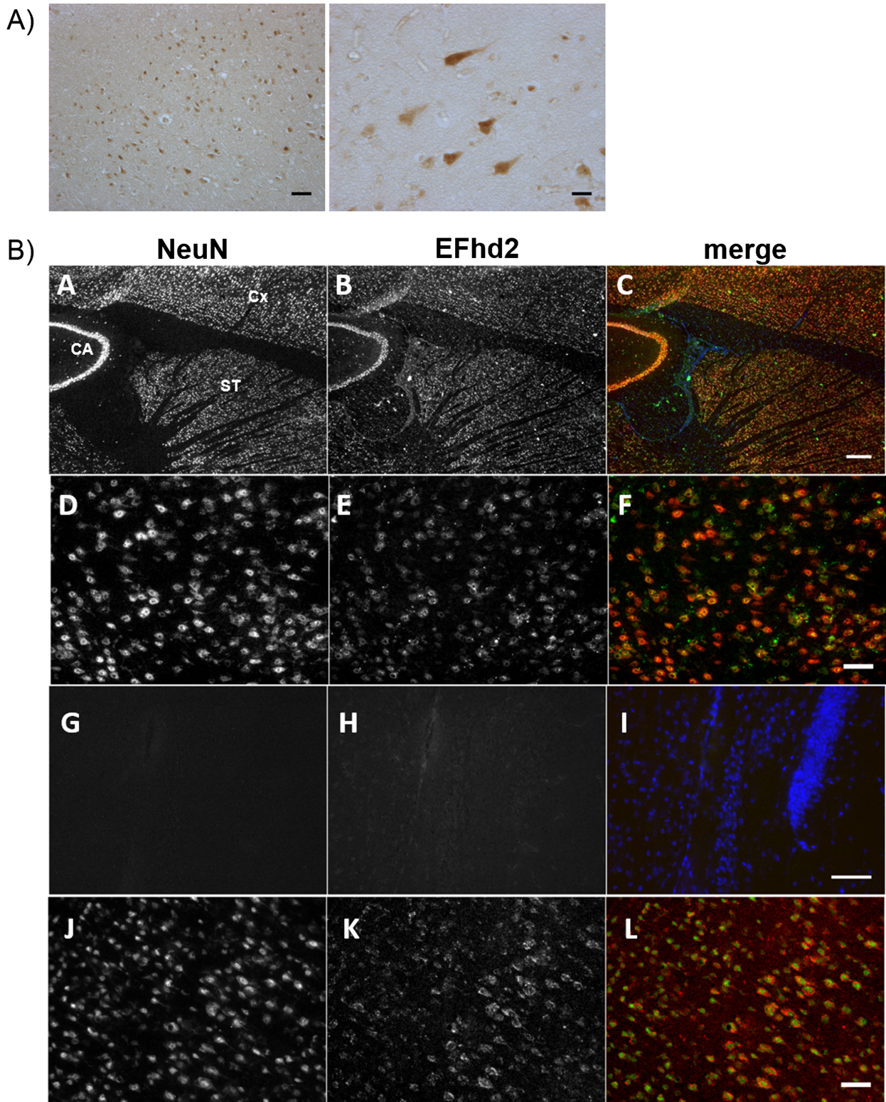
FIGURE 4. (I) Immunohistochemistry (IHC) with a rabbit polyclonal antibody (RbpAb) on human brain tissues for EFhd2. Scale bars = 100 μm (left); 50 μm (right). (II) IHC on mouse brain for NeuN (red: A, D, G, J ), EFhd2 with a goat polyclonal antibody (green: B, E, H ), and merge ( C, F, I ). ( A–C ) EFhd2 is present in neuronal layers of the hippocampus (cornu ammonis [CA]), cortex (Cx), and subcortical structures (striatum [ST]). Scale bar = 250 μm. ( D–F ) Expression in the frontal cortex is restricted to anti-NeuN-labeled neurons. Scale bar = 50 μm. ( G–I ) No primary antibody, merge with 4',6-diamidino-2-phenylindole. Scale bar = 100 μm. ( J–L ) Similar results were obtained using an RbpAb against an N-terminal epitope of EFhd2 stained in the frontal cortex (red). Scale bar = 50 μm.
