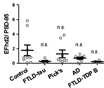
FIGURE 5. EFhd2 protein levels in the frontal cortex are reduced in total homogenates from patients with dementia but not in synaptoneurosomes. (A) Western blots showing EFhd2 protein levels in human frontal cortex tissue extracts from nondemented controls and individuals with Alzheimer disease (AD), frontotemporal lobar degeneration (FTLD)-tau (FTLD-tau), Pick disease, or FTLT-TDP Type B (FTLD-TDP). Beta-actin was used as a loading control for homogenates and nonsynaptic fractions; PSD-95 was used as a loading control for synaptoneurosomes fractions. (B) Quantification of EFhd2 protein bands by densitometry. Error bars = SEM. Homogenate: 1-way ANOVA, p = 0.0301 ; * p < 0.05 compared with control by using Dunnett post hoc test. Synaptoneurosomes: 1-way ANOVA, p = 0.1108 . Nonsynaptic: 1-way ANOVA, p = 0.4848 .
