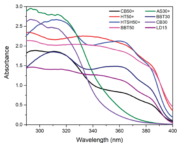
Fig. 10 Absorbance spectra of the sunscreen samples, AS30+ and CB30 show low absorbance in the UVA range, which indicates poor UVA radiation protection of these samples.
