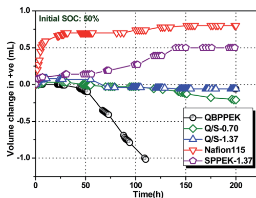
Fig. 6 The static water transport volume of membranes.
