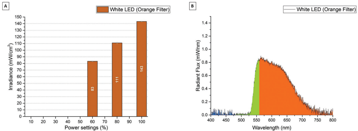
Fig. 5: A) Irradiance (mW/cm 2 ) for the Zeon Endeavour XL TrueColor White LED with the Orange blue light blocking filter in the different power settings. B) Spectral Radiant Flux (mW/nm) for the Zeon Endeavour XL TrueColor White LED with the Orange blue light blocking filter in the max (100 %) power setting.
