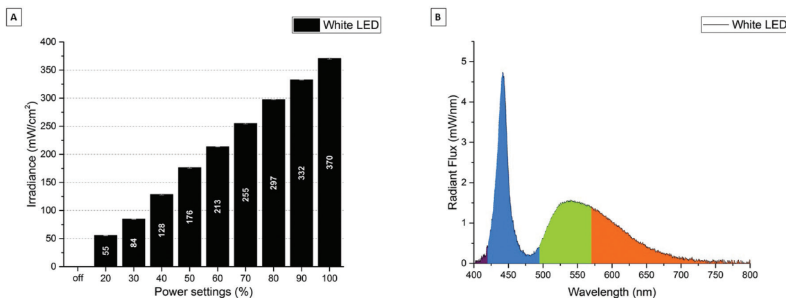
Fig. 2: A) Irradiance (mW/cm 2 ) for the Starlight Nano3 White LED in the different power settings. B) Spectral Radiant Flux (mW/nm) for the Starlight Nano3 White LED in the max (100 %) power setting.
