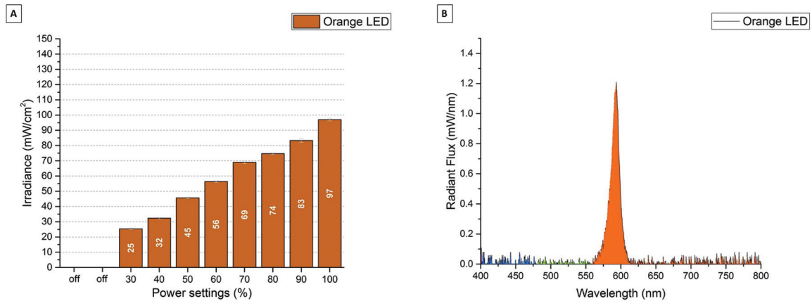
Fig. 4: A) Irradiance (mW/cm 2 ) for the Starlight Nano3 Orange LED in the different power settings. B) Spectral Radiant Flux (mW/nm) for the Starlight Nano3 Orange LED in the max (100 %) power setting.
