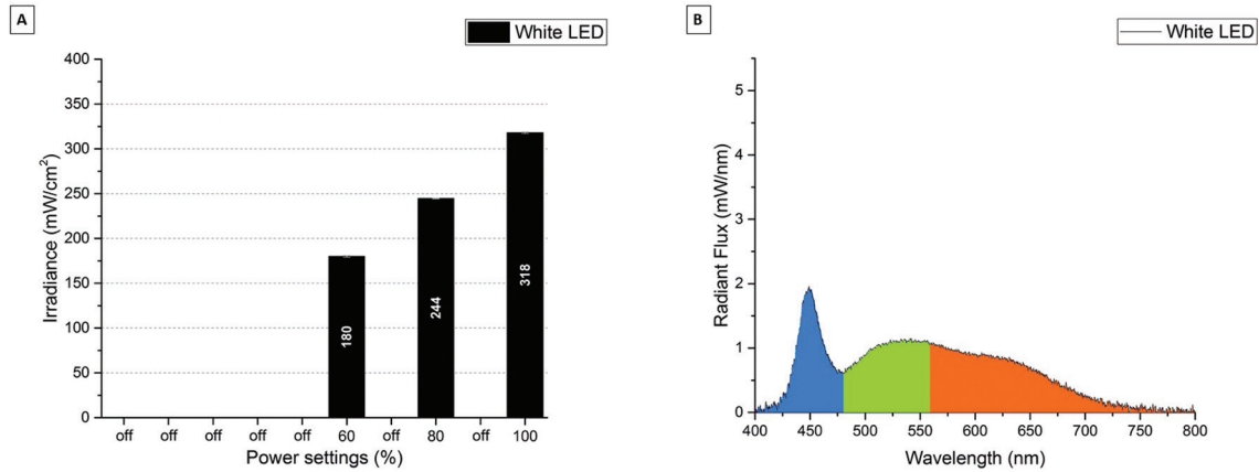
Fig. 3: A) Irradiance (mW/cm 2 ) for the Zeon Endeavour XL TrueColor White LED in the different power settings. B) Spectral Radiant Flux (mW/nm) for the Zeon Endeavour XL TrueColor White LED in the max (100 %) power setting.
