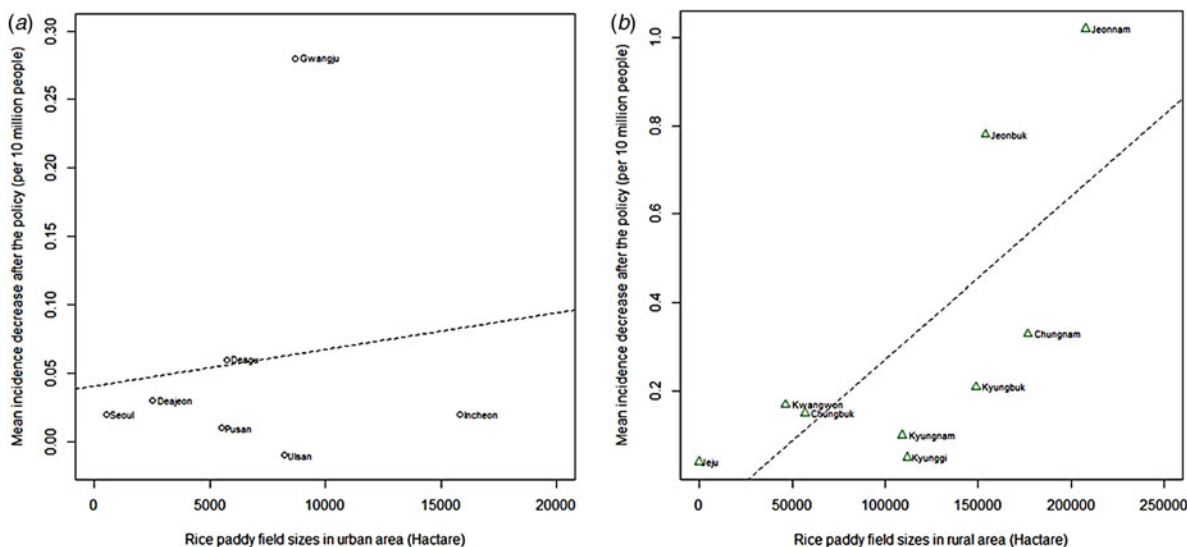
Fig. 2. Association between rice paddy field areas and the decrease in human leptospirosis incidence in metropolitan cities and provinces. This figure shows the decrease in leptospirosis in urbanized metropolitan cities (a) and provinces (b). The level of decrease on leptospirosis incidence in metropolitan cities is relatively smaller with no significant association with rice paddy field areas ( r = 0.11, P = 0.82 ). The level of decrease on leptospirosis incidence in provinces is bigger than metropolitan cities and has a significant association with the rice paddy field areas ( r = 0.82, P < 0.01 ).
