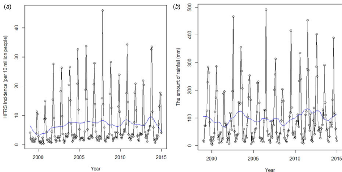
Fig. 3. The environmental drivers of leptospirosis. (a) The incidence (solid line with circle) and trend of HFIRS (a proxy of exposure to rodents; solid line without circle). There was no significant change with HFIRS during study period ( RR = 1.15, P = 0.06 ). (b) The amount of rainfall (solid line with circle) and its trend (solid line without circle). There was no significant differences between pre- and post-period of Livestock Manure Control Act enforcement ( P = 0.97 ).
