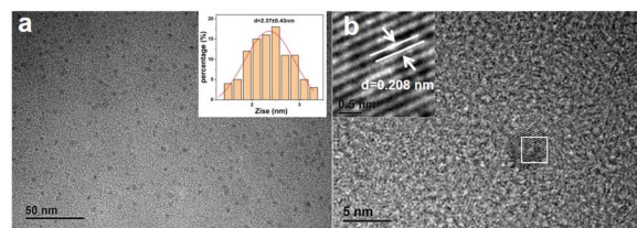
Fig. 3 (a) The TEM image of the WCS-CDs (inset: the particle size distribution); (b) the HRTEM image of the WCS-CDs.
