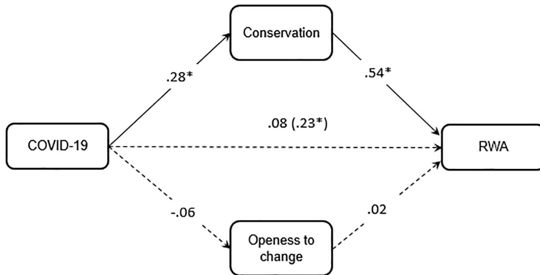
Fig. 1. Mediation model. Note. RWA = Right-Wing Authoritarianism. Parameter coefficients are standardized. Total effect is indicated in parentheses. * p < .001 .
