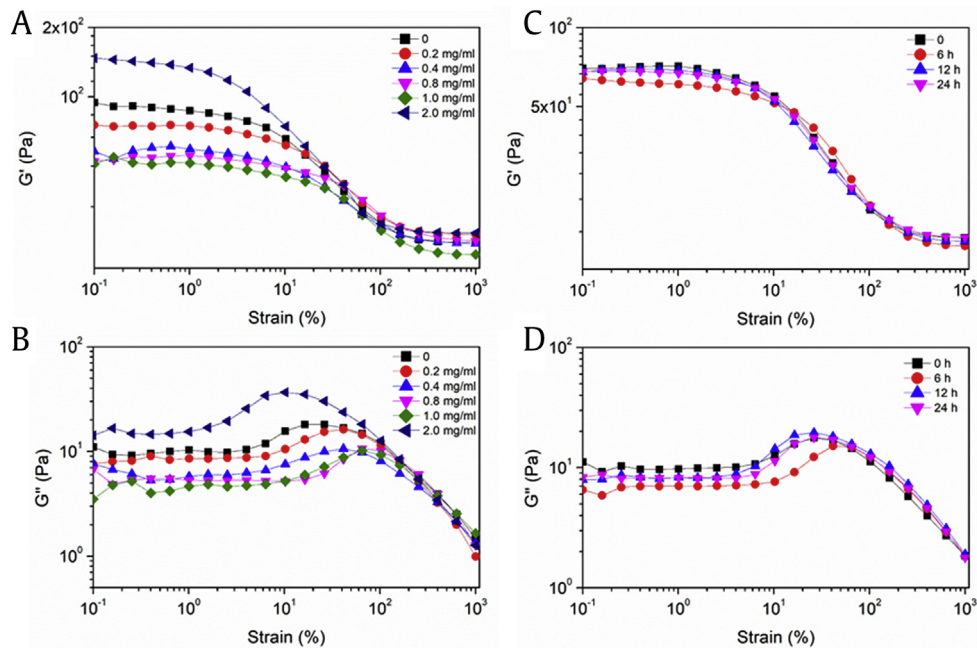
Fig. 7. Log profile of strain-dependent storage modulus ( G' ) and loss modulus ( G'' ) for the skin equivalent. (A) G' and (B) G'' curves according to red ginseng concentration. (C) G' and (D) G'' curves according to treatment duration at 0.8 mg/mL red ginseng.
