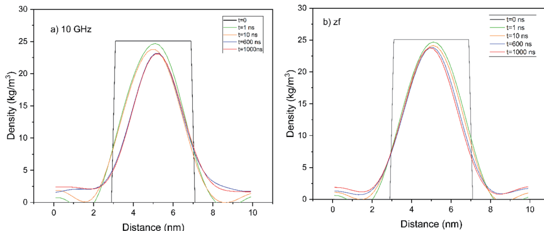
Fig. 4 The development in time of parabolic-like spatial H 2 -concentration profiles along the laboratory x -direction sampled from NEMD simulation, in accord with analytic theory of unsteady-state diffusion of a gaseous guest from a solid. 25 Under the influence of (a) 10 GHz electromagnetic field, and (b) zero-field conditions.
