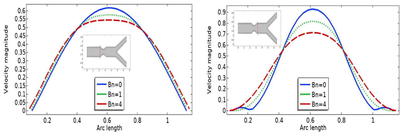
Figure 7. Velocity profile for different Bn .
