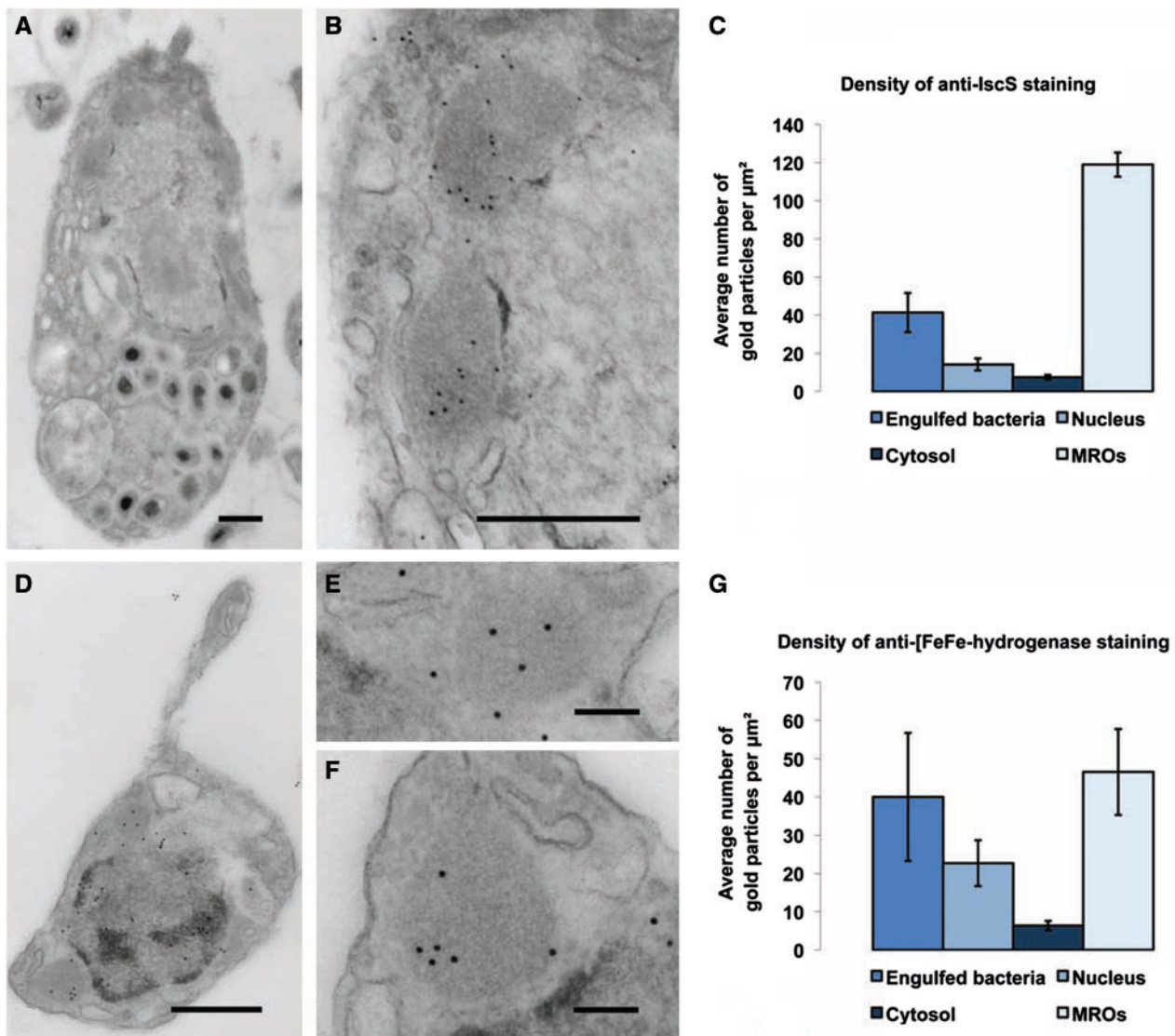
FIG. 3. Immunogold localization of IscS and [FeFe]-hydrogenase in S. incarcerata cells. (A) A representative whole cell fixed for immunogold staining; scale bar, 500 nm; this image has been cropped in order to show only the whole cell from which the insets shown were derived. (B) Magnified section from the cell pictured in (A), showing gold particles corresponding to anti- Giardia IscS localization; scale bar, 500 nm. (C) Mean density of immunogold labeling in engulfed bacteria, the cytosol, the nucleus, and MROs (seven cells), \pm standard error of the mean. (D) Representative whole cell fixed for immunogold staining; scale bar, 500 nm; this image has been cropped in order to show only the whole cell from which the insets shown were derived. (E, F) Magnified sections from the cell pictured in (A), showing gold particles corresponding to anti- Mastigamoeba [FeFe]-hydrogenase localization; scale bar, 500 nm. (G) Mean density of immunogold labeling in engulfed bacteria, the cytosol, the nucleus, and MROs (13 cells), \pm standard error of the mean. Brightness and contrast have been adjusted in each image to enhance visibility of the mitochondria and gold particles.
