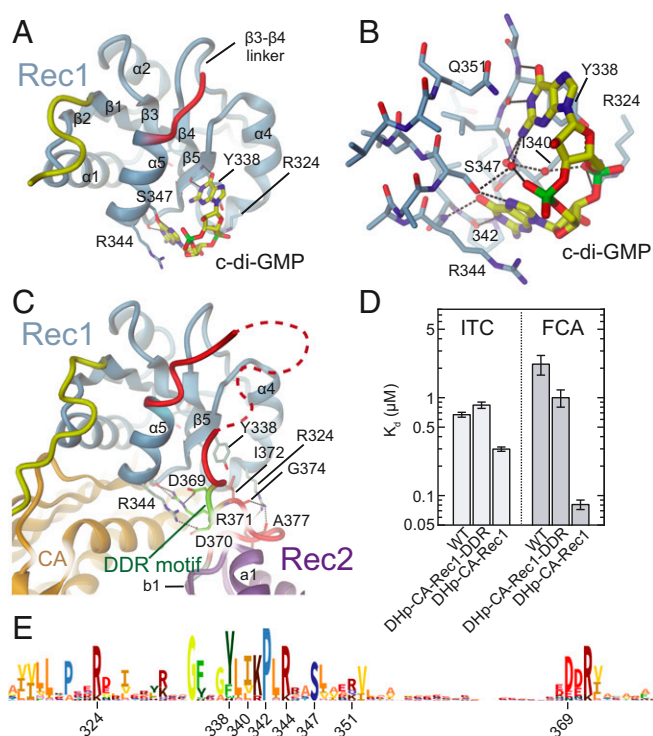
Fig. 3. C-di-GMP and Rec1-Rec2 linker compete for Rec1 binding. ( A and B ) Crystal structure of ShkA Rec1 in complex with c-di-GMP with interacting residues shown in full. The Watson–Crick edges of both guanines form H-bonds with Rec1 main-chain atoms. The bases stack with Y338, Q351 and with R344. The hydroxyl of S347 is H-bonded to a guanine N7 group. Both Y338 and R324 interact with 1 of the phosphates. See also SI Appendix , Fig. S4 . ( C ) Structure of Rec1 of full-length ShkA in same orientation as ShkA Rec1 in A . The comparison shows that the DDR motif (light-green) is bound to the same site on Rec1 as c-di-GMP (for a superposition see SI Appendix , Fig. S4B ). Note that R324 and R344 of Rec1 are involved both in c-di-GMP and linker binding. ( D ) C-di-GMP binding to various ShkA constructs as measured by ITC (Upper) and FCA (Lower). Construct DHp-CA-Rec1 shows a significantly lower dissociation constant compared to the other variants, which can be attributed to the absence of the competing DDR segment. Full data are given in SI Appendix , Fig. S5 . ( E ) Sequence logo encompassing the c-di-GMP binding site of the ShkA Rec1 domain.
