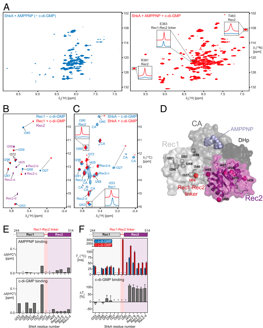
Fig. 2. C-di-GMP binding to ShkA leads to release of the Rec2 domain. (A) Two-dimensional [ 15 N, 1 H]-TROSY spectra of ShkA/AMPPNP (blue spectrum) and ShkA/AMPPNP/c-di-GMP (red spectrum). The Insets show 1D [ 1 H]-cross sections for representative amide protons. (B) Overlay of 2D [ 13 C, 1 H]-HMQC spectra of the isolated [ 13 C/ 1 H δ1 -Ile]Rec1 domain in apo state (blue) and c-di-GMP-bound state (red), and the isolated [ 13 C/ 1 H δ1 -Ile]Rec2 domain (purple). (C) Spectral overlay of 2D [ 13 C, 1 H]-HMQC spectra of [ 13 C/ 1 H δ1 -Ile]ShkA in apo state (blue) and c-di-GMP-bound state (red). The 2 Insets show 1D [ 1 H]-cross sections for representative methyl protons. Sequence-specific resonance assignments of the \delta 1 methyl groups are either indicated or assigned to the Rec2 or CA domain. (D) Crystal structure of ShkA/AMPPNP. Surface representation of the monomer composed of 4 domains: DHp (dark gray), CA with bound AMPPNP (gray), Rec1 (light gray), and Rec2 (purple). The \delta 1 methyl groups of isoleucine residues in the Rec1 and Rec2 domains are shown as spheres together with I372 (red sphere) that is part of the Rec1-Rec2 linker. (E) Chemical shift perturbation of isoleucine \delta 1 methyl groups upon addition of AMPPNP to ShkA ( Upper ) and upon addition of c-di-GMP to ShkA/AMPPNP ( Lower ). (F) Transverse relaxation times of isoleucine \delta 1 methyl carbons of ShkA/AMPPNP (blue bars) and ShkA/AMPPNP/c-di-GMP (red bars). The Lower panel shows the relative change of T_2 ( 13 C) upon addition of c-di-GMP ( \Delta T_2 ). (E and F) Asterisks indicate methyl groups that are either not assigned or line-broadened beyond detection in at least 1 of the 2 states.
