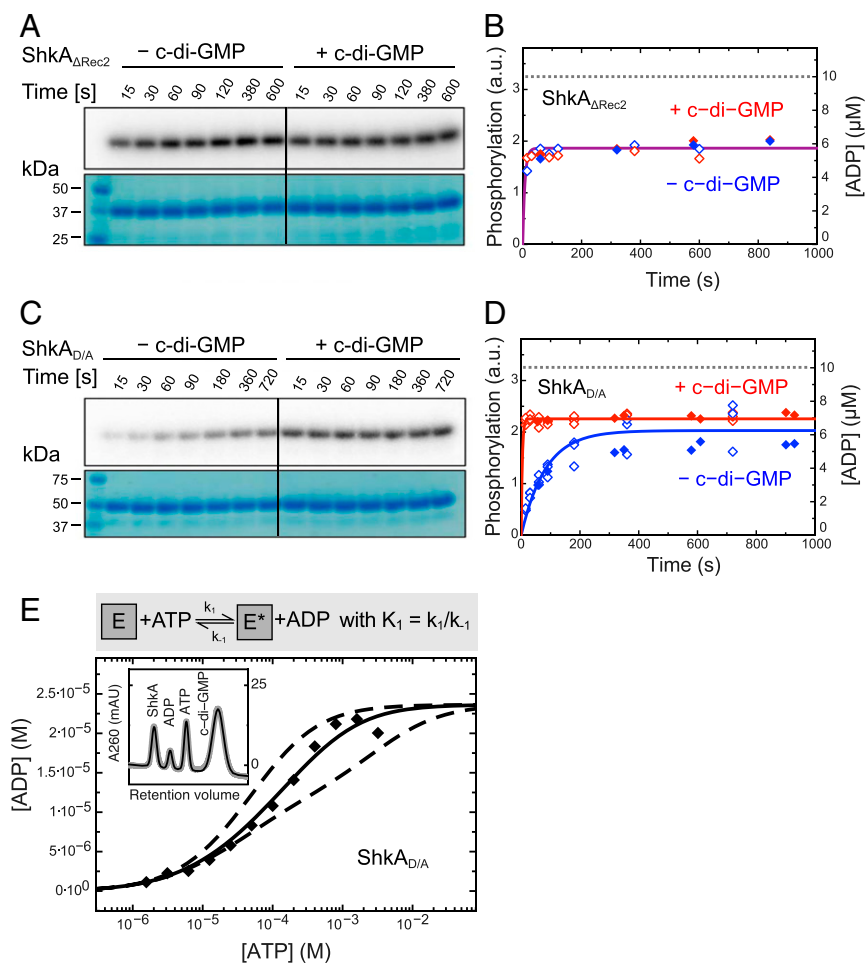
Fig. 5. ShkA autophosphorylation is reversible and, in the presence of Rec2, controlled by c-di-GMP. (A and C) ShkA _{\Delta\text{Rec}2} and ShkA _{\text{D/A}} phosphorylation after indicated times of incubation as measured by autoradiography using [ \gamma - ^{32}\text{P} ]-ATP, in the absence and presence of c-di-GMP as indicated. SDS/PAGE gels are shown below and indicate equal loading. For additional data, see SI Appendix, Fig. S7A . (B and D) Time course of ShkA _{\Delta\text{Rec}2} and ShkA _{\text{D/A}} phosphorylation (hollow symbols) and ADP production (filled symbols), in the absence (blue) and presence (red) of c-di-GMP. Phosphorylation values were calculated from the band intensities in A and C; ADP concentrations were determined by oIEC. Solid lines represent exponential fittings of the autoradiograph data [for ShkA _{\text{D/A}} : k_{1, \text{c-di-GMP}} = (0.012 \pm 0.002)\text{s}^{-1} ]. The dashed line indicates the employed enzyme concentration. (A–D) [ShkA variant]: 10 \mu\text{M} , [c-di-GMP]: 25 \mu\text{M} , [ATP]: 200 \mu\text{M} . (E) Equilibrium concentration of ADP as a function of initial ATP concentration as determined by oIEC. [ShkA _{\text{D/A}} ]: 20 \mu\text{M} , [c-di-GMP]: 50 \mu\text{M} . The continuous line is the fit of the simple reversible, noncooperative bi-bi reaction shown on the top to the data with K_1 = k_1/k_{-1} = 0.13 and a refined [ShkA _{\text{D/A}} ] of 23 \mu\text{M} , (see also SI Appendix, Methods ). Reactions with positive or negative cooperativity would yield the dashed curves (calculated with equilibrium constants for second phosphorylation event of 1.3 and 0.013, respectively) that do not fit the data. (Inset) Representative oIEC chromatogram.
