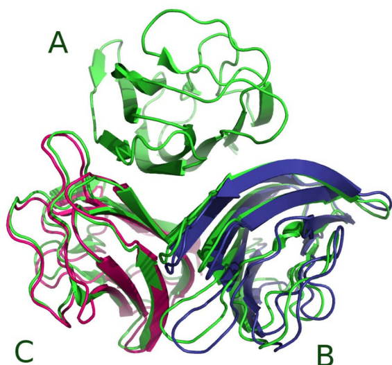
Figure 2 CIq system. (PDB: 1PK6) The crystallographic system is represented in green. Units B (in blue) and C (in magenta) were obtained after the 3-body docking strategy (see text).
