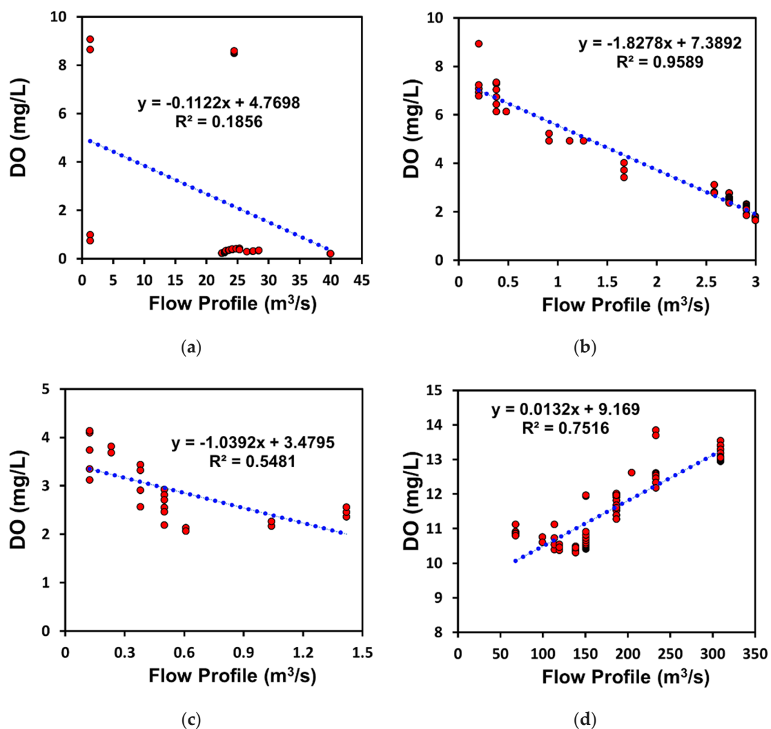
Figure 10. Dissolved oxygen concentration with respect to flow profile (a) Yamuna River, (b) Baghmati River, (c) Galing River, and (d) Nakdong River.
