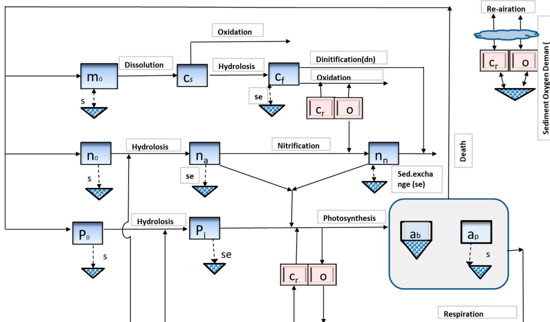
Figure 3. QUAL2Kw graphical illustration of water quality parameters: o—dissolved oxygen, ap—phytoplankton, ab—algae (bottom algae), n0—nitrogen (organic), Mo—detritus, Cf—C-BOD fast, Cs—C-BOD slow, Cr—inorganic carbon, nn—nitrite nitrogen, na—ammonium nitrogen, pi—inorganic phosphorus, and p0—organic phosphorus.
