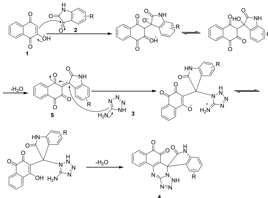
Scheme 2. A suggested pathway for the formation of the hybrid.
