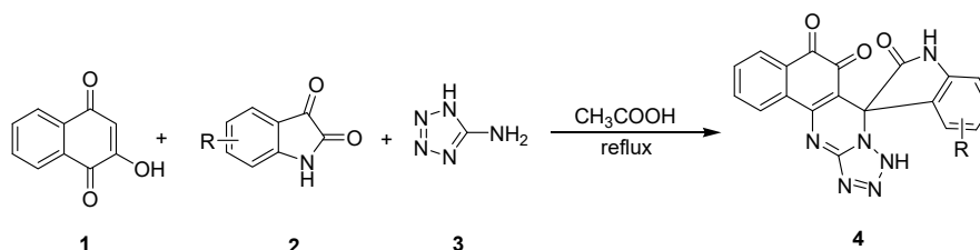
Scheme 1. Synthesis of spirooxindole- O -naphthoquinone hybrids.
