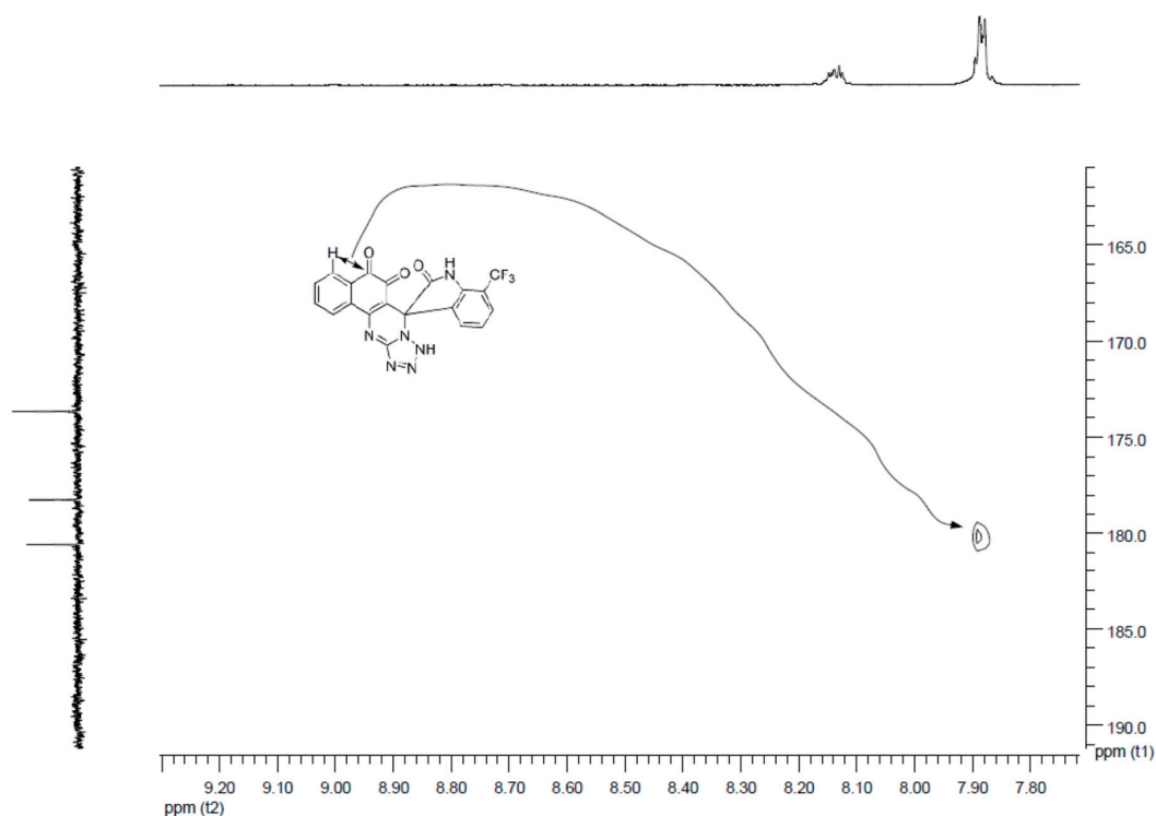
Figure 2. Locally amplified HMBC of 4n.
