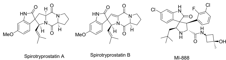
Figure 1. Spirooxindoles with anticancer activities.
