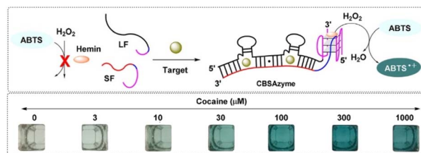
Fig. 2 Working mechanism and the chromogenic catalysis performance of the CSBAzyme. Reprint from ref. 43, with permission. Reprinted (adapted) with permission from Anal. Chem. , 2019, 91 (11), 7199–7207. Copyright 2019 American Chemical Society.
