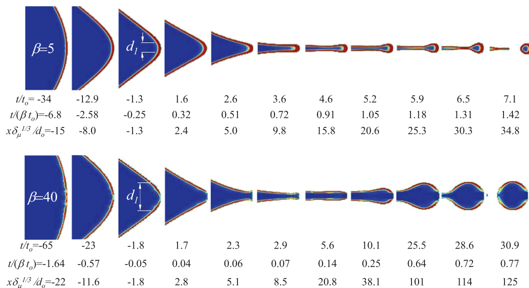
Figure 3. Images of the droplet ejection obtained from simulations with \beta = 5 and \beta = 40 , and \delta_\mu = 1.6 . The time was referenced to the instant when v = v_o . The colors indicate the dimensionless volume charge density \hat{q}/(\epsilon_o E_o d_o^{-1}) from 0 (blue) to 1 (red). Around t/(\beta t_o) \sim -0.3 , the surface charge density reaches its maximum value at a circumference with diameter d_1 . Beyond this stage, the tip moves faster than the bulk ions. The conical collapse up to t/t_o \sim 3.2 is geometrically self-similar.
